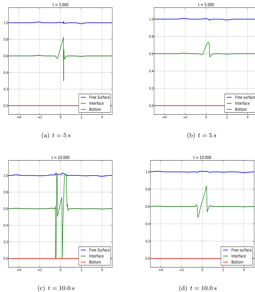
Fig. 5.10: Test 2: Free surface and interface evolution. Roe scheme (left column). Roe scheme with artificial viscosity (right column).
