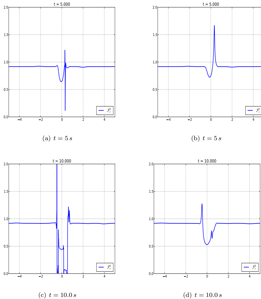
Fig. 5.12: Test 2: Stability number \mathcal{F}_r . Roe scheme (left column). Roe scheme with artificial viscosity (right column).
