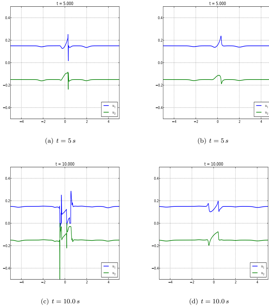
Fig. 5.11: Test 2: Velocities of the two layers. Roe scheme (left column). Roe scheme with artificial viscosity (right column).
