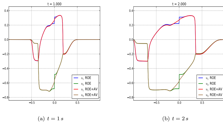
Fig. 5.8: Test 1: Velocities at each layers: comparison between Roe scheme (blue and green lines) and Roe with artificial viscosity (red and brown lines).
