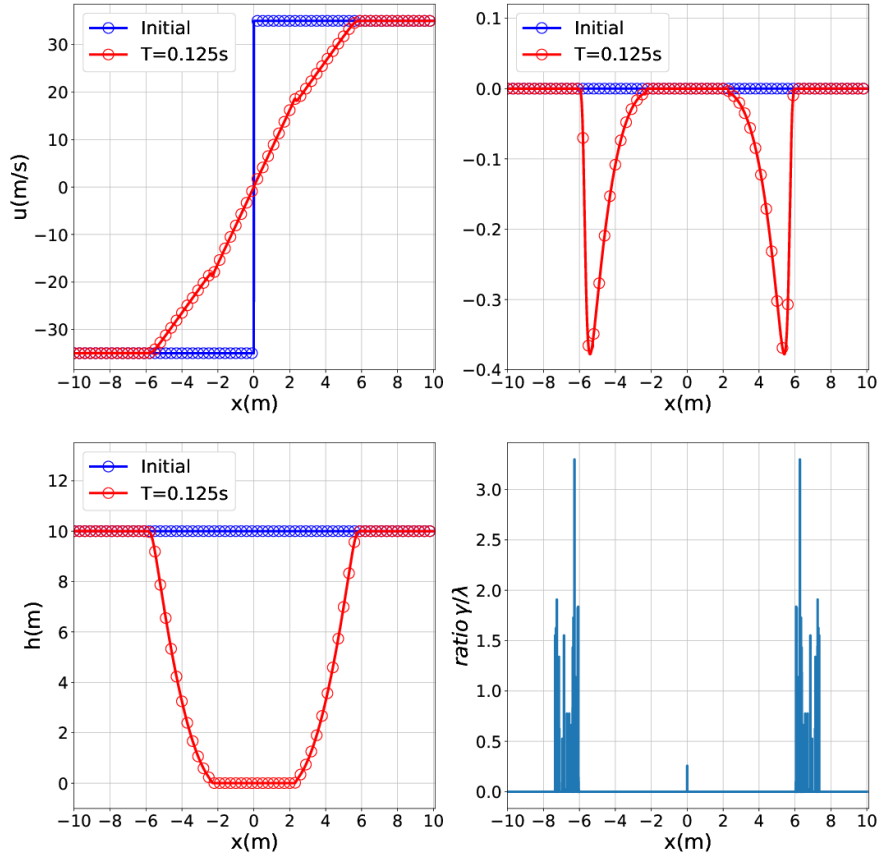
Fig. 5.6: Space variations at the final time T = 0.125s of the velocity height (upper-left), energy budget (upper-right) and water height (lower-left), together with the ratio \gamma/\lambda (lower-right) Mesh size: 10 000 cells.
