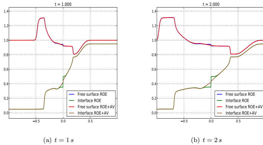
Fig. 5.7: Test 1: Free surface and interface: comparison between Roe scheme (blue and green lines) and Roe with artificial viscosity (red and brown lines).
