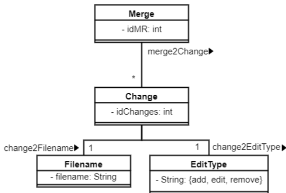
Figure 4: Collaborative version control platforms Meta model – Part 2
