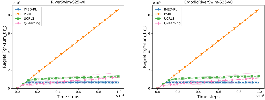
Figure 4: Average regret and quantiles (0.1 and 0.9) curves of algorithms on a standard communicating 25-states RiverSwim (left), and in its ergodic version (right).
