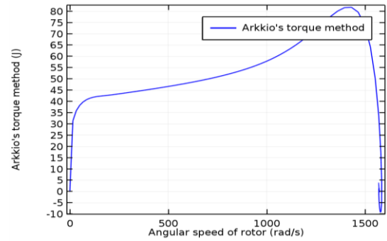
Fig.9b. Speed-Torque characteristics at f=500\text{Hz}
