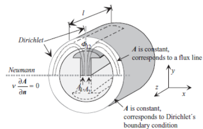
Fig.1. Definition of boundary conditions
