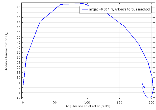
Fig.9a. Speed-Torque characteristics at f=50\text{Hz}
