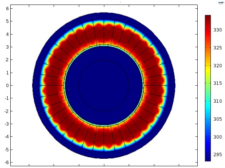
Fig.6a. Surface temperature (K) at f=50Hz
