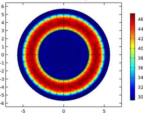
Fig.6b. Surface temperature (K) at f=500Hz
