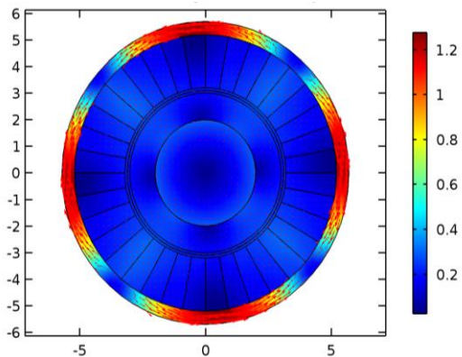
Fig.4b. Surface Magnetic flux density in the material (T) at f=500Hz
