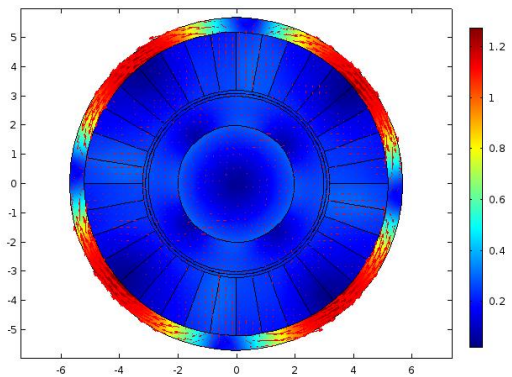
Fig.4a. Surface Magnetic flux density in the material (T) at f=50Hz
