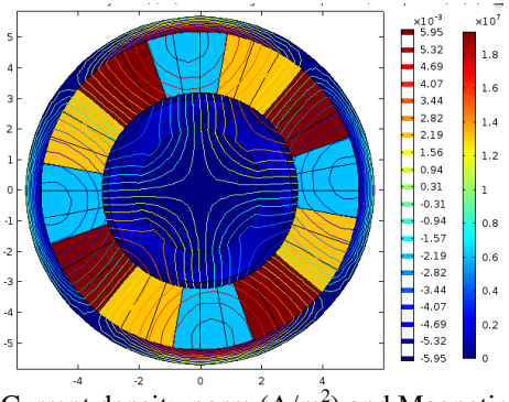
Fig.5a. Current density norm ( A/m^2 ) and Magnetic vector potential, z component (Wb/m) at f = 50Hz
