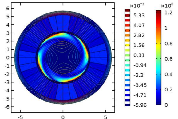
Fig.5b. Current density norm ( A/m^2 ) and Magnetic vector potential, z component (Wb/m) at f = 500Hz
