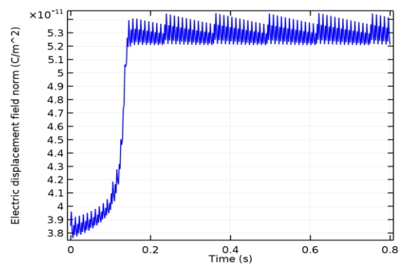
Fig.10a. Electric displacement, D ( \text{C}/\text{m}^2 ) in stator core at f=500\text{Hz}
