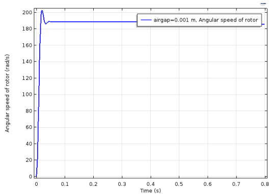
Fig.8a. Angular speed of rotor (rad/sec) at f=50\text{Hz}
