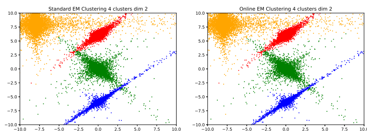
Figure 12: Standard EM (Left) vs online EM (Right) clustering result.
