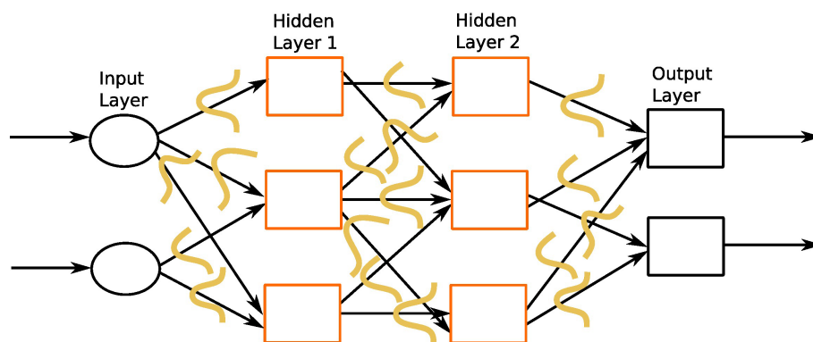
FIGURE 8 An instance of Bayesian regularized neural network with one input layer, two intermediate hidden layers, and one output layer. The orange curves represent prior distribution on each weight connection.
