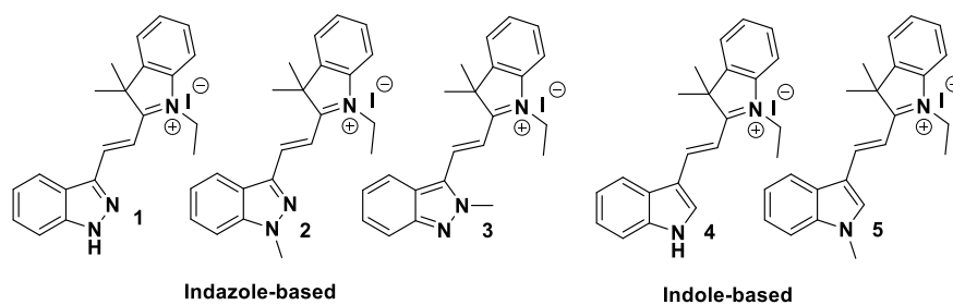
73 Fig. 1. Structures of indazole and indole merocyanines.
