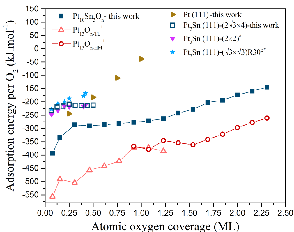
Figure 2. Average adsorption energy (kJ mol -1 ) plotted against oxygen coverage (ML) on Pt 10 Sn 3 /Al 2 O 3 . The calculated adsorption energies of oxygen on Pt (111), Pt 3 Sn (111) and Pt 13 /Al 2 O 3 are also presented from previous works: + Sangnier et al. [12] and # Dupont et al. [24] The reported adsorption energies taken from Ref [24] which were expressed per atomic oxygen, are therefore multiplied by a factor two to be compared with other values.
