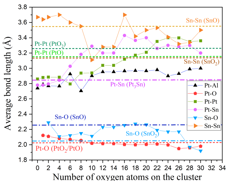
Figure 3. Averaged Pt-Al, Pt-O Pt-Pt, Pt-Sn, Sn-O and Sn-Sn bonds length (Å) as a function of the number of adsorbed oxygen atoms. The maximal bond lengths were set to 3.0 Å for Pt-Al, 2.5 Å for Pt-O, 3.8 Å for Pt-Pt, 3.8 Å for Pt-Sn and 2.5 Å for Sn-O. Dotted red, dotted dark green, dash dotted light blue and dash dotted purple lines correspond to the Pt-O, Pt-Pt, Sn-O and Pt-Sn bond lengths in PtO 2 and SnO 2 bulk phases, respectively. Dotted light green, dotted red, dash dotted dark blue line correspond to the Pt-Pt, Pt-O and Sn-O bond lengths in PtO and SnO bulk phases, respectively.
