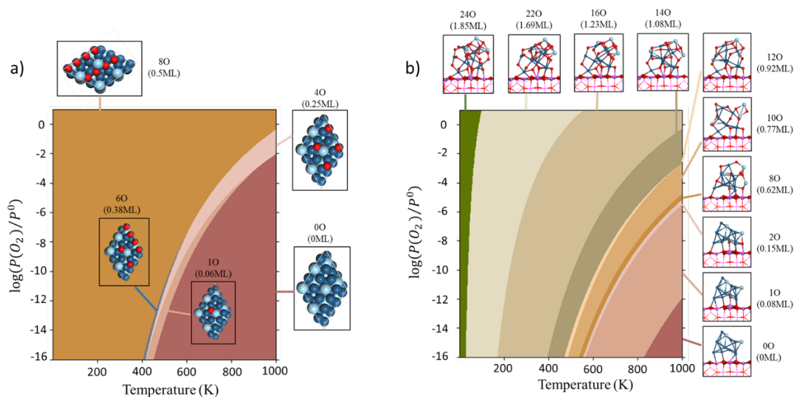
Figure 6. a) Thermodynamic phase diagram depicting the most stable oxygen coverage as a function of temperature (K) and the O 2 partial pressure (bar) for a) Pt 3 Sn (111) and b) Pt 10 Sn 3 /Al 2 O 3 (100). The structures of the systems exhibiting a significant stability domain are also depicted with top views for a) and side views for b). Color code for the atomic structures is the same as in Figure 1.
