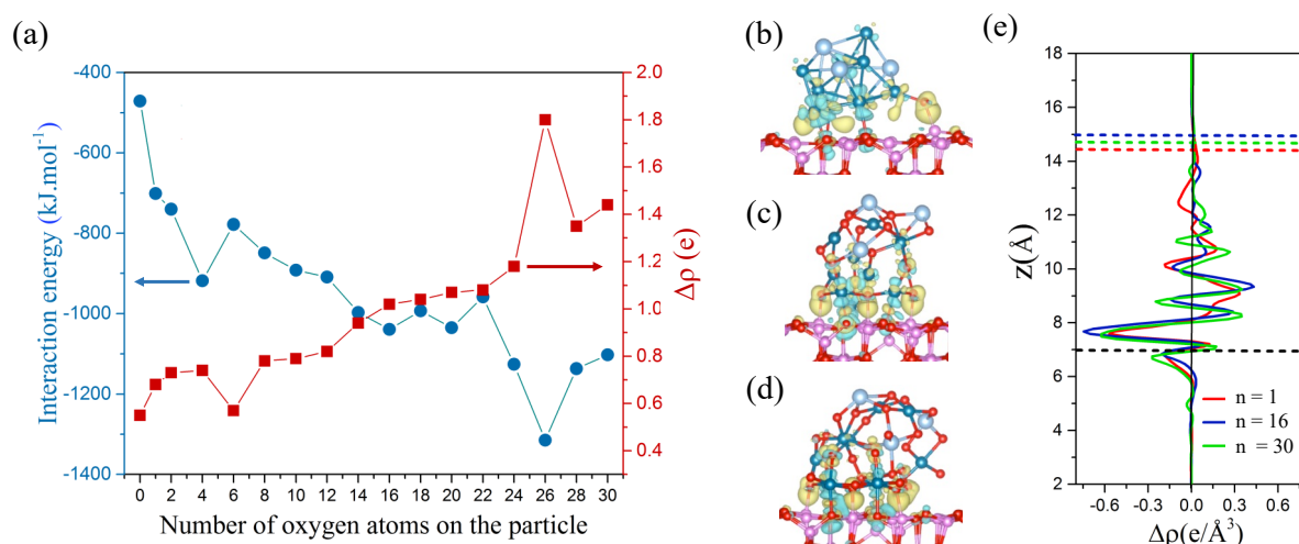
Figure 4. (a) Evolution of the interaction energy between the alumina support and the oxidized platinum-tin clusters and the Bader charge transfer from alumina surface to \text{Pt}_{10}\text{Sn}_3\text{O}_n cluster).
