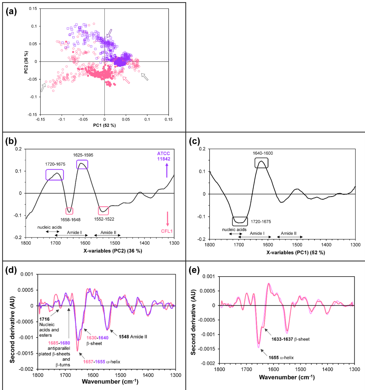
Fig.6 Principal Component Analysis (PCA) of processed FTIR spectra in the 1800 – 1300 \text{cm}^{-1} region, of L. bulgaricus CFL1 bacteria (pink circles, freeze-sensitive) and L. bulgaricus ATCC 11842 bacteria (purple squares, freeze-resistant) acquired using the ATR-FTIR inverted microscope (open symbols, one to two cells) and using the transmission FTIR microscope (full symbols, clusters of a few thousands of cells) (a-c), and second derivatives (d-e) of selected points indicated by arrows in (a).
