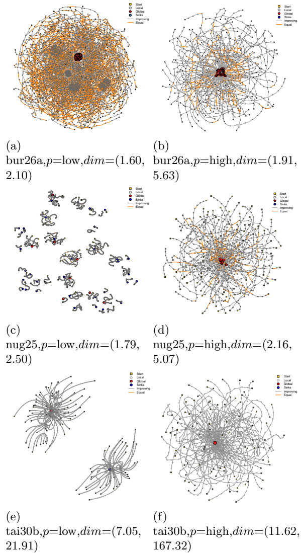
Fig. 1: Monotonic LONs for selected instances and the two perturbation strengths, p = low (left) p = high (right). The median and maximum fractal dimension are also indicated in the sub-captions as dim = (\text{median}, \text{maximum})
