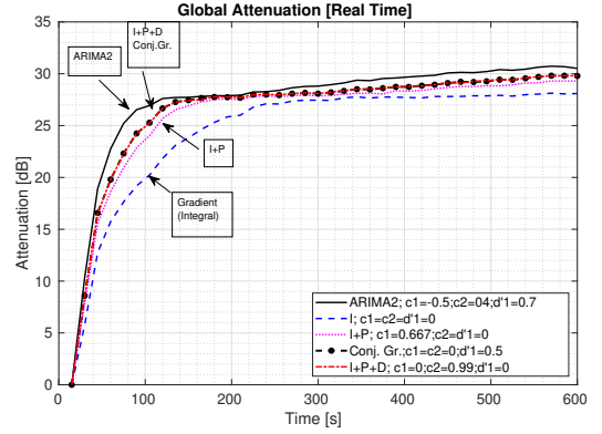
Fig. 6. Time evolution of the global attenuation for the algorithms of Table I.
