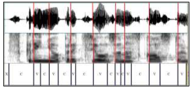
Figure 1: Spectrogram and manual annotation of the Italian utterance “scrigno prezioso nascosto” (from 2001 sample).
