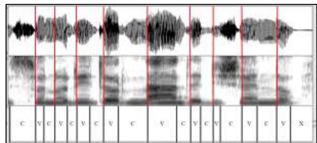
Figure 2: Spectrogram and manual annotation of the Italian utterance “sono ritornate dicendo” (from 2007 sample).
