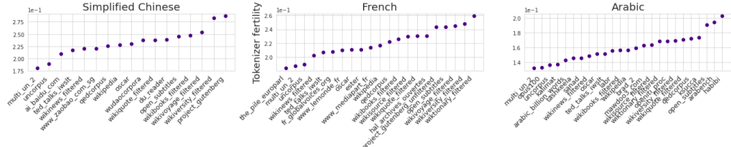
Figure 8: Tokens per byte for each French, Simplified Chinese, and Arabic component for tokenizers trained on this corpus. Lower values mean the component (X axis) is more similar in aggregate to the rest of the corpus.
