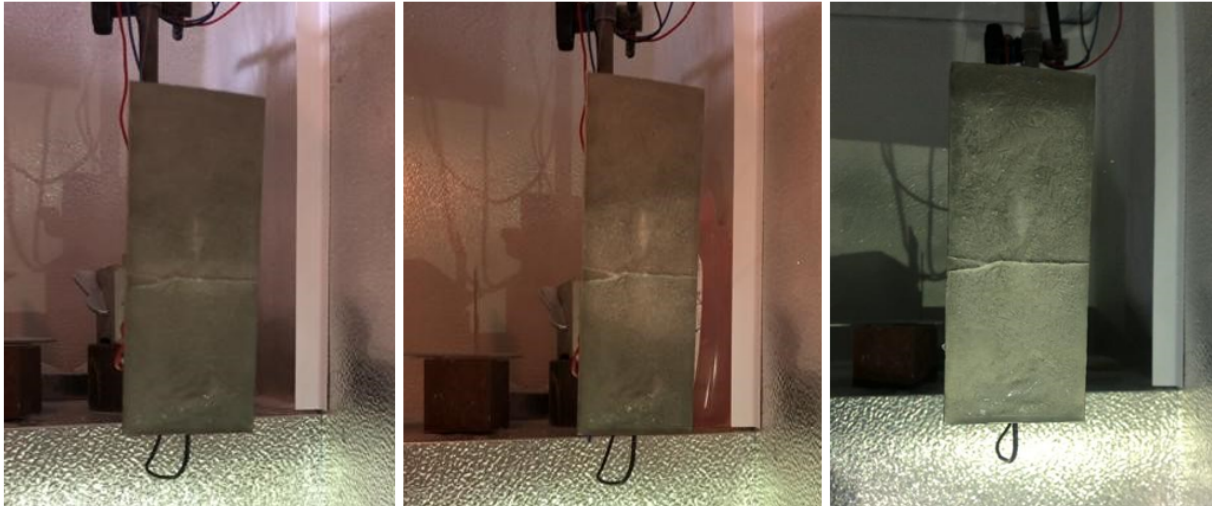
Figure 10 – Example of adhesive propagation with a long ice block using first mode of bending and increasing voltage (150 V, 200 V and 250 V)
