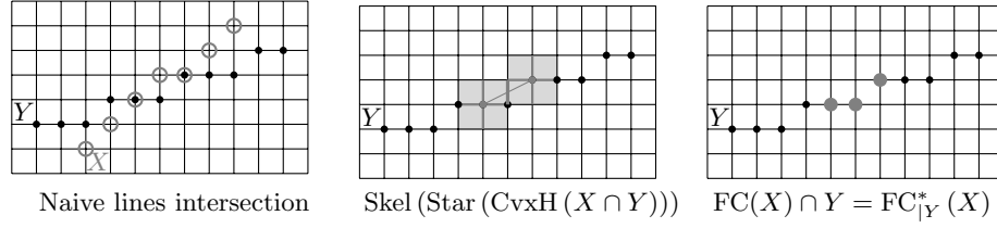
Fig. 2. Relative fully convex envelope for naive lines having disconnected intersection.
