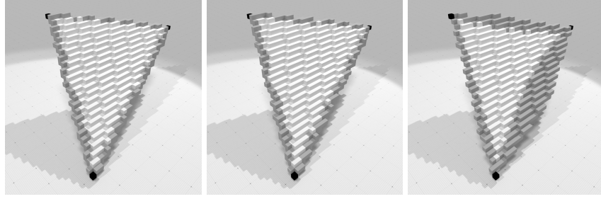
generic faces \sharp \mathcal{T}^* = 1193 standard faces \sharp \mathcal{T}_1^* = 985 naive faces \sharp \mathcal{T}_\infty^* = 567
