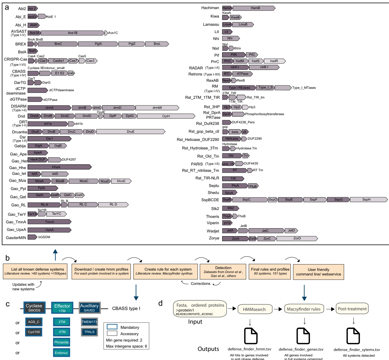
Fig. 1 DefenseFinder, a tool to detect all known prokaryotic antiviral systems. a List of systems included in DefenseFinder. Systems are ordered alphabetically. For systems with several types, each system is represented by one type and other types are indicated in parentheses (Full list, Supplementary Data Table 1). b Workflow for the creation of DefenseFinder. c Example of a DefenseFinder rule (in the MaccyFinder syntax) for the detection of system CBASS type I. Cyclase and effector proteins are mandatory while the sensing protein is only accessory. This means the system allows for it to be missing in a detected CBASS type I system. Different profiles are recognized for a protein. ex cyclase (SMODS, AGC_C, Cyc100). d DefenseFinder function layout. DefenseFinder takes an ordered multifasta protein file. A search for specific HMM profiles is conducted, the MacSyfinder rules specific for antiviral systems are applied on the search results, generating three results files.
