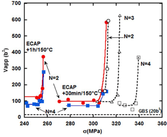
Fig. 9. The apparent activation volume of the alloy processed by ECAE (scaled in b^3 ) as a function of the applied stress. Open marks: as deformed. Full marks: ECAE and aging at 150^\circ\text{C} .
