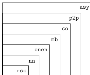
(a) The hierarchy of MSC classes.
