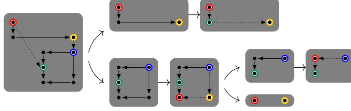
Figure 13: Decomposition game for the MSC of Fig. 3b. This is a 3-winning game for Eve.
