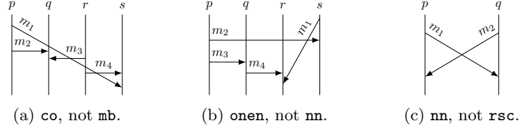
Figure 7: Examples of MSCs for various communication models.
