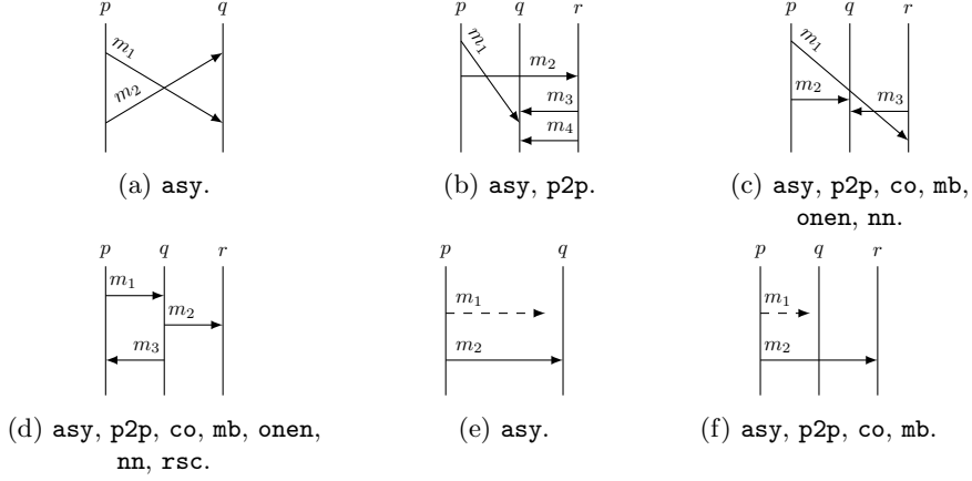
Figure 3: Examples of MSCs for various communication models.
