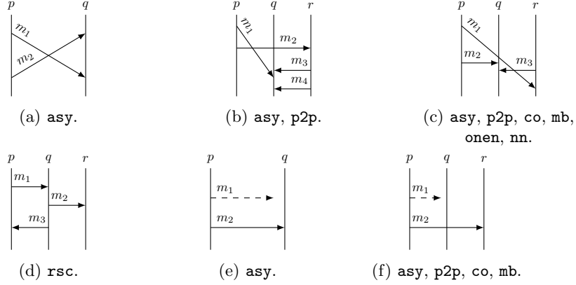
Figure 3: Examples of MSCs for various communication models.
