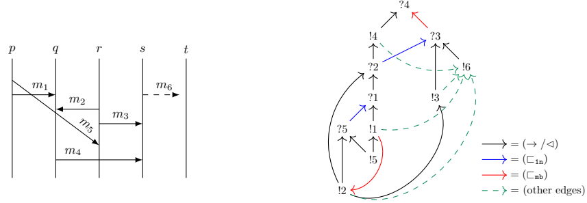
Figure 5: An MSC and its EDG. In the EDG, only meaningful edges are shown.
