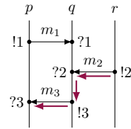
Figure 1: An example of MSC. Red arrows denote a causal path.
