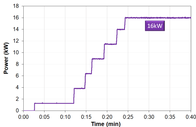
Figure 6: The beam power up to 16 kW proton beam.
