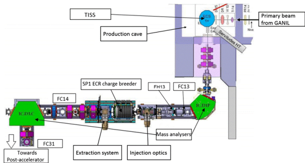
Figure 7: The SPIRAL1 for production of 1^+ radioactive ion beams with the possibility of charge breeding in the ECR booster before post acceleration in the CIME cyclotron.
