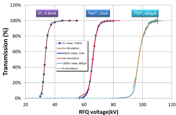
Figure 4: Transmission in the RFQ of the three reference Q/A.
