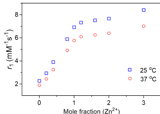
Figure 1. Relaxometric titration of GdL 2 (1 mM) with \text{Zn}^{2+} at 7 T at 25 °C and 37 °C in PBS (pH 7.4).
