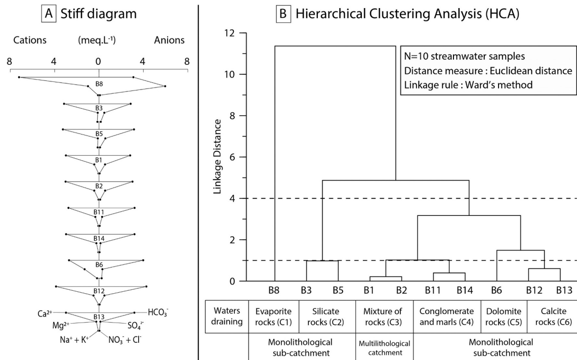
Fig. 2. Comparison of the chemical patterns using the Stiff diagram (A) and hierarchical clustering analysis (B) of the streamwater chemical composition of the different sites for the spatial sampling campaign. The drainage bedrocks are mentioned for each cluster of sites.
