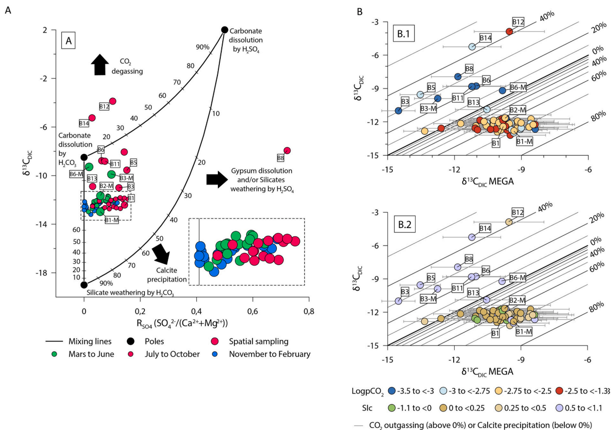
Fig. 5. (A) Relationships between \delta^{13}\text{C}_{\text{DIC}} and R_{\text{SO}_4} ( \text{SO}_4^{2-}/(\text{Ca}^{2+} + \text{Mg}^{2+}) ), showing the influences of the different processes. End-member compositions as described in the text are shown to illustrate that most of the waters are distributed along a mixing line. The black arrows indicate possible reasons for the deviations from these mixing lines. Values from 10 to 90 over the mixing lines represent the potential contribution percentage of each end member for each dot. Nomenclature of 4 sites sampled in March 2019 ends with “-M” (B) Relationships between the \delta^{13}\text{C}_{\text{DIC}} signature measured in streamwaters ( \delta^{13}\text{C}_{\text{DIC}} ) and the \delta^{13}\text{C}_{\text{DIC}} value calculated using the geochemical discrimination ( \delta^{13}\text{C}_{\text{DIC}} MEGA): (B1) according to the \text{pCO}_2 and (B.2) to the Saturation Index of calcite (SIC). The uncertainties (horizontal grey lines) are due to the isotopic signature of carbonate rocks. Straight black lines represent theoretical processes of \text{CO}_2 outgassing (above theoretical line 0%) and carbonate precipitation (under theoretical line 0%), according to the end-members compositions represented in Fig. 5.A (for further details, see Supplementary Information B Table B4).
