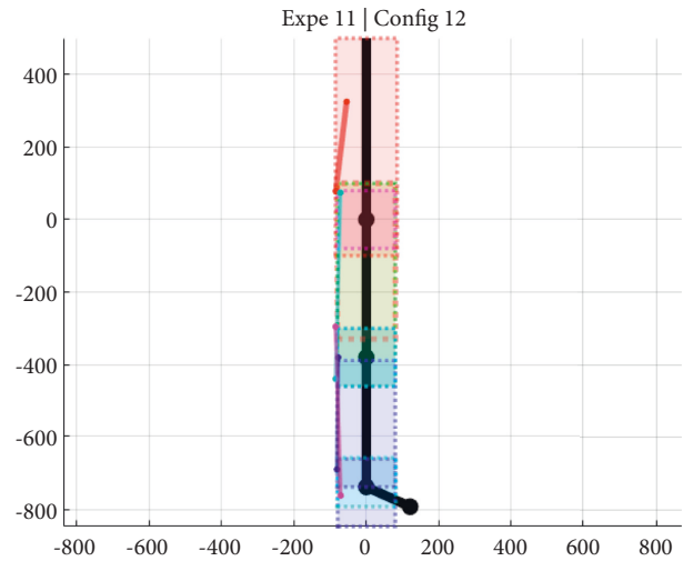
FIGURE 21: Optimal versatile geometry for architecture 12.
