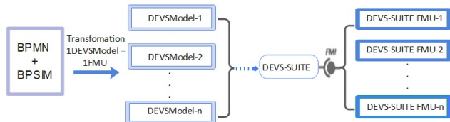
Figure 5. Transformation from BPMN+BPSIM to FMUs
