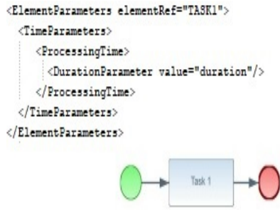
Figure 2. BPMN task extended with BPSIM duration
