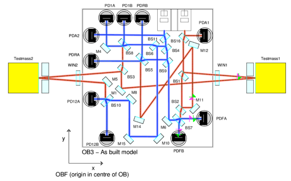
FIG. 2. Top panel: The four interferometers on the OB. The Optical Bench Frame (OBF) has its origin in the center of the OB. Bottom panel: Schematic overview of the OMS and its main components (reprint from [1] for convenience).
