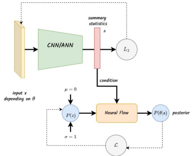
Figure 30. Illustration of a Neural Flow for estimating posterior distributions. This type of approach is starting to become common in simulation based inference approaches for estimating cluster masses or cosmological parameters. A first Neural Network with a standard L_2 loss is used to obtain some summary statistics of the data which are then use as a condition for a Neural Flow mapping a simple distribution into an approximation of the posterior.
