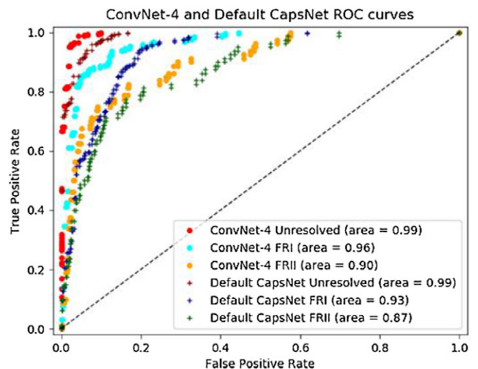
Figure 5. Comparison of Capsule Networks and CNNs applied to classify morphologies of radio galaxies. The ROC curves show the different performances. Capsule Networks do not offer a significant gain in this context. Figure adapted from Lukic et al. (2019)
