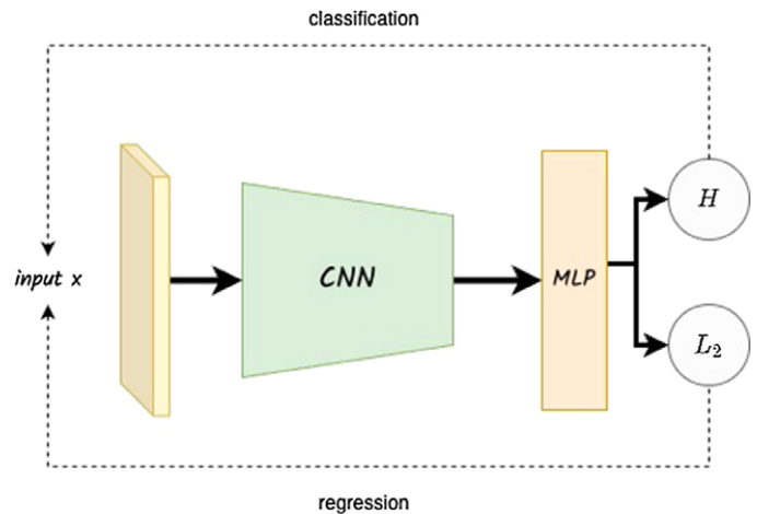
Figure 3. Schematic view of a simple Vanilla type Convolutional Neural Network, the most common approach for binary, multi-class classification and regression in extragalactic imaging. The input, which is typically an image is fed to a series of convolutional layers. The resulting embedding is used as an input of a Multi-Layer Perceptron which outputs a float or array of floats. If the problem is a classification, the standard loss function is the cross-entropy ( H ), while if it is a regression the quadratic loss ( L_2 ) is usually employed.
