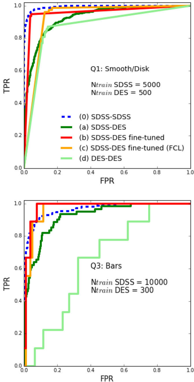
Figure 7. Example of Transfer Learning adapted to galaxy morphological classification exploring how to use a CNN trained on SDSS to the DES survey. Each panel shows a different morphological feature (smooth/disk, bars from top to bottom). The different lines show the ROC curves using different training models and test sets. The work concludes that when using a small subset of DES galaxies to refine the weights of a CNN trained on SDSS, the accuracy of the classification becomes optimal (red solid lines compared to blue dashed lines). Figure adapted from Domínguez Sánchez et al. (2019)
