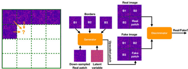
Figure 42. Sequential generation and upsampling strategy of the scalable GAN for N-body modelling presented in Perraudin et al. (2019a) scaling up to 256^3 . The left illustration shows how the sequential generation of a large volume would proceed. The right plot illustrates the proposed architecture where the generator is conditioned on both neighbouring patches, and on the lower resolution patch, which at sampling time would be generated by a separate GAN trained on coarser volumes. Distribute under the Creative Commons CC BY licence ( http://creativecommons.org/licenses/by/4.0/ ).
