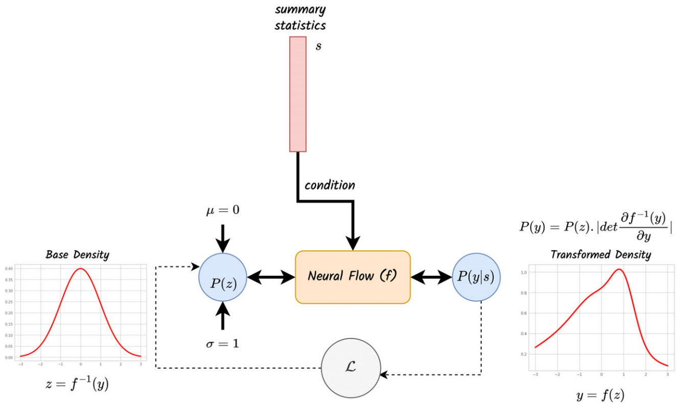
Figure 19. Illustration of a Normalising flow. This density estimator model is used to transform a simple distribution (typically a Normal distribution) into a more complex density using an invertible function f parametrised by a neural network which is optimised by maximising the log likelihood. The transformation can also be conditioned to an additional set of parameters ( s in the figure).
