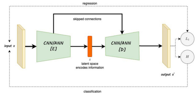
Figure 12. Schematic representation of a Unet type of architecture. This is typically used for addressing image to image problems (e.g. segmentation, galaxy properties in 2D). A first CNN (encoder) encodes information into a latent space ( z ), which is then fed to another CNN (decoder) which produces an image. One particularity of the Unet is the presence of skipped connections between the encoding and decoding parts which have been demonstrated to provide higher accuracies.
