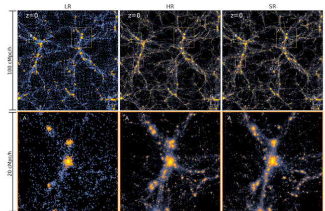
Figure 41. Illustration of N-body simulation super-resolution from Li et al. (2020a) showing from left to right, the Low-Resolution (LR) input, High-Resolution (HR) target, and Super-Resolution output of the model. The bottom row is a zoom-in on the region marked A.
