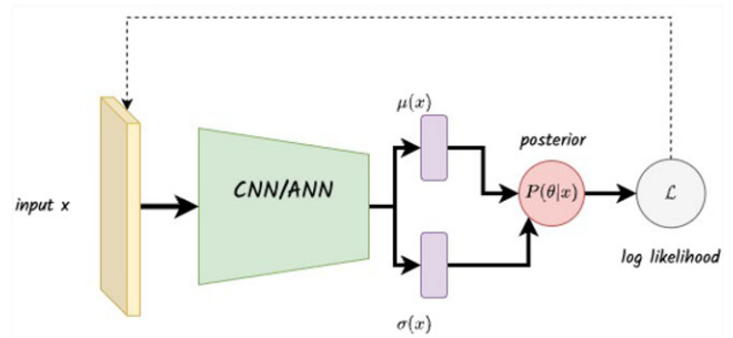
Figure 20. Representation of a Mixture Density Network (MDN). It is a generalisation of a standard CNN/ANN in which the output has been replaced by a probability distribution parametrised with some parameters ( \mu , \sigma in the figure). MDNs provide an estimation of the random (aleatoric) uncertainty. The loss function is the generalised log likelihood.
