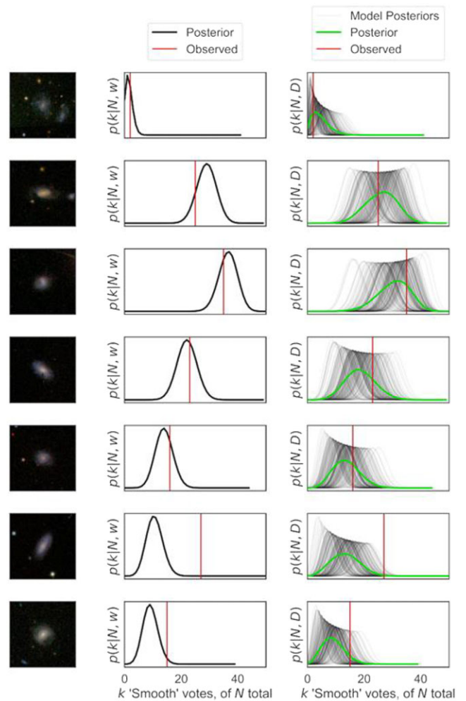
Figure 6. Example of posterior distributions of morphologies estimated from the votes of different classifiers. The leftmost column shows an image of a galaxy. The middle column shows the posterior predicted by a single network (black), while the right column shows the posterior averaged over 30 Monte Carlo dropout approximated networks. The red vertical lines indicate the ground truth value, which generally shows a good overlap with the posterior distribution. Figure adapted from Walmsley et al. (2020)
