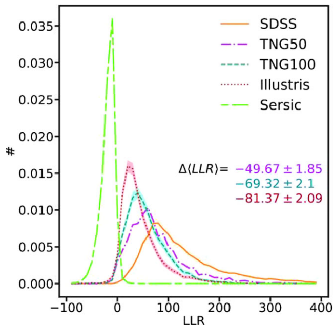
Figure 38. Distribution of likelihood ratios obtained with two pixelCNN networks of observations (SDSS) and different models as labelled. The closer the histograms from simulations are to the one from SDSS, the more realistic the simulation is. The unsupervised model is able to capture the improvement of simulations with time. Figure from Zanisi et al. (2021).
