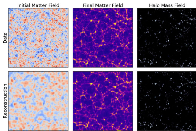
Figure 43. Illustration of an application of differentiable neural mapping between the dark matter density and dark matter halo fields from Modi et al. (2018). The top row shows the initial conditions dark matter field, final dark matter field (at z=0 ), and the dark matter halo field obtained by a FoF halo finder. The bottom row shows the result of a reconstruction by gradient descent of these initial conditions, using a neural network to provide the mapping between the final density field and the halo field.
