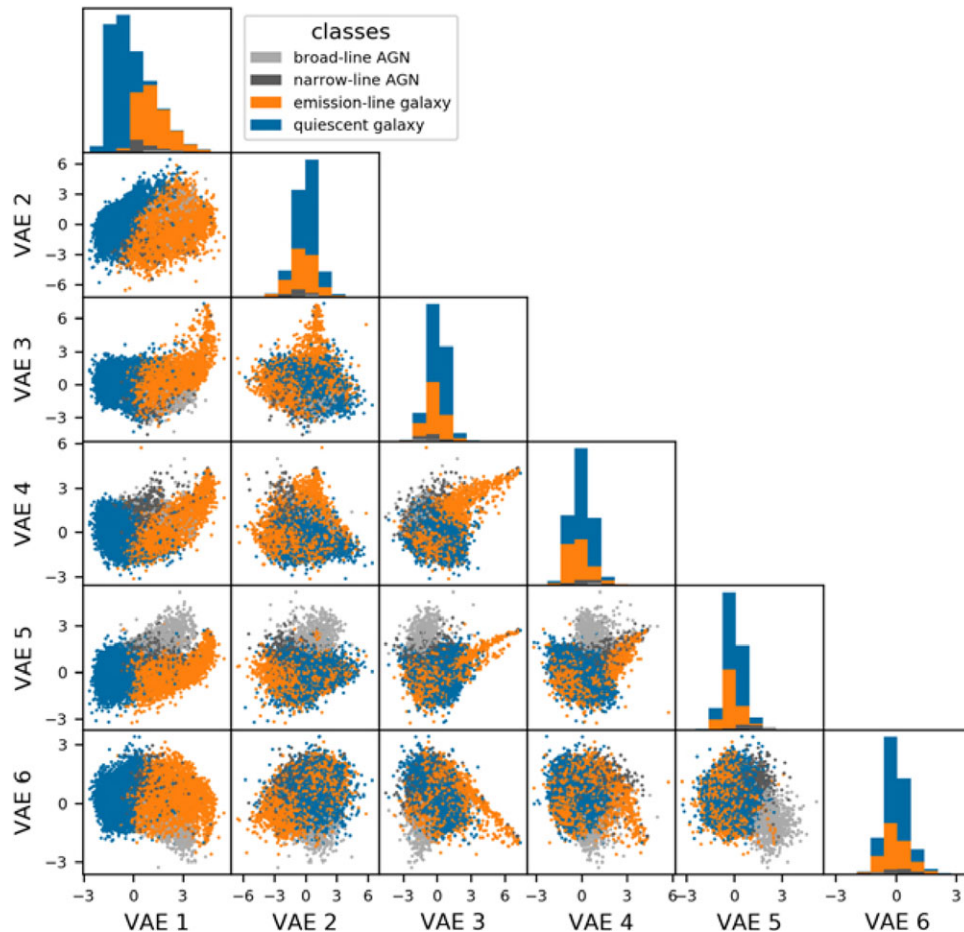
Figure 32. Variational Autoencoder for dimensionality reduction and data visualisation. The figure show how the different types of spectra (labelled with different colours) populate different projections of the latent space. Figure adapted from Portillo et al. (2020)
