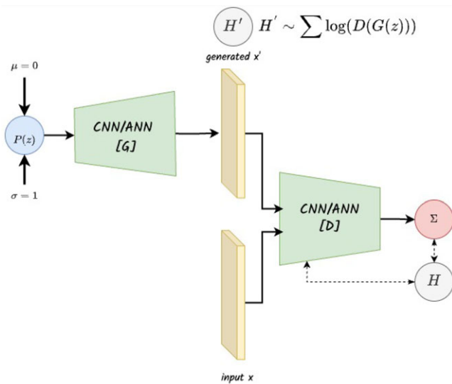
Figure 16. Schematic representation of a standard Generative Adversarial Network (GAN). It has been used as a generative model for deblending, identifying outliers as well as for accelerating cosmological simulations among others. A first CNN (generator) maps a random variable into an image, which is then fed to a second CNN (discriminator) together with real images to distinguish between both datasets. The generator and discriminator networks are trained alternatively.
