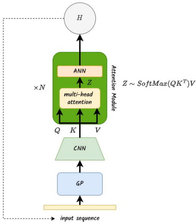
Figure 10. Example of typical transformer architecture for the classification of light curves. A Gaussian Process is first used to homogenise the time sampling and the resulting sequence is fed into a CNN for feature extraction. The attention modules are used to extract the final features which are used to classify.
