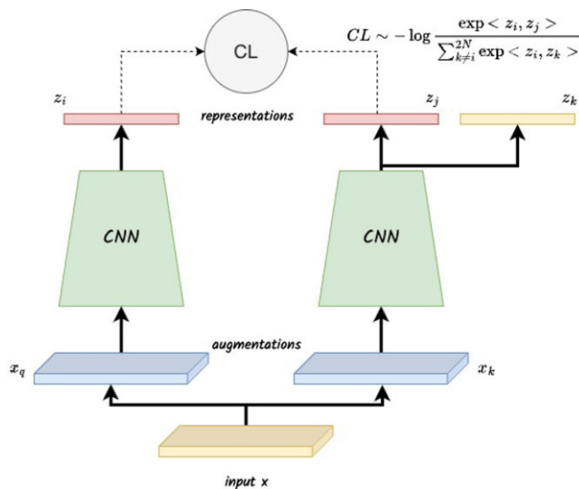
Figure 33. Illustration of a self-supervised contrastive learning architecture. Multiple random augmentations of the same image (positive pairs) are fed to two different CNNs which map them into a latent representation space. Also during training, pairs of completely different images (negative pairs) are also fed to the two CNNs. The contrastive loss is optimised to increase (decrease) the dot product of representations of positive (negative) pairs. Contrastive learning is starting to be used for dimensionality reduction and as a generalised feature extraction process for multiple downstream tasks such as galaxy classification or photometric redshift estimation.
