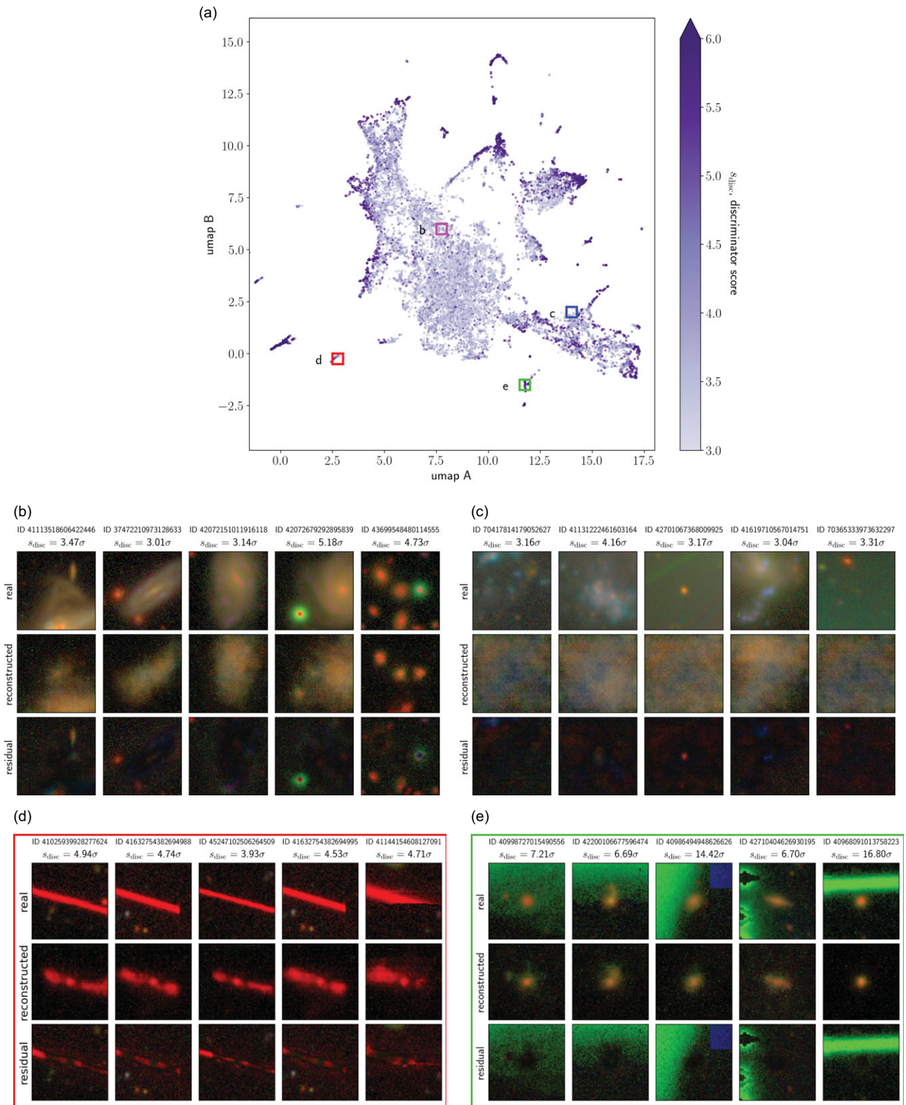
Figure 37. Example of anomalous objects identified with a combination of WGAN and a CAE applied to the HSC survey. The top panel shows the latent space from the image residuals of the WGAN reconstruction obtained with the CAE. The images below show examples of different regions of the parameter space. Figure from Storey-Fisher et al. (2021).
