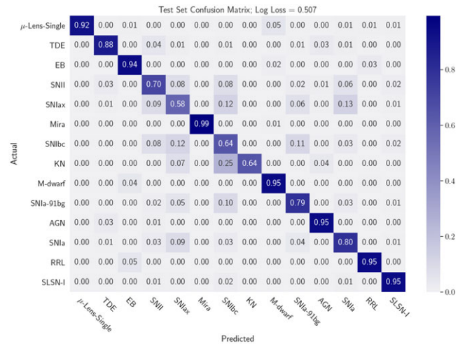
Figure 11. Transformer applied to SN photometric light curve classification. The figure shows a confusion matrix on the PLAsTiCC simulated dataset. Most of the classes are identified with accuracies larger than 90% as seen in the diagonal of the matrix. Figure adapted from Allam & McEwen (2021)
