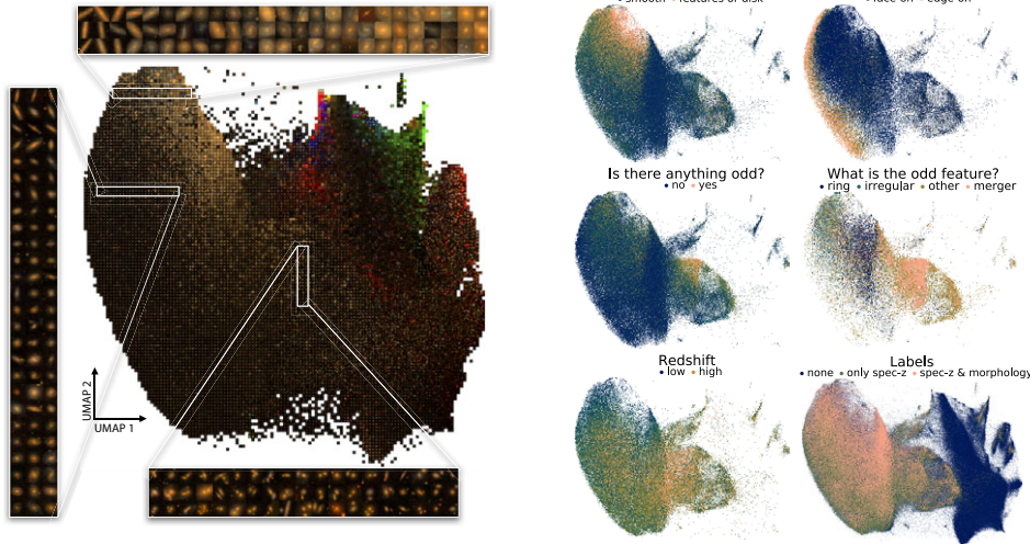
Figure 34. Self-supervised learning applied to multi-band SDSS images. The left panels shows a UMAP of the representations obtained with contrastive learning. The panels on the right show the same UMAP colour coded with different galaxy properties. Similar images are clustered together. Figure adapted from Hayat et al. (2021).
