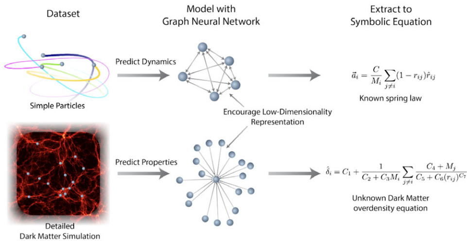
Figure 39. Cartoon illustrating the method to extract physical equation from a deep learning model applied to different datasets. Figure from Cranmer et al. (2020).
