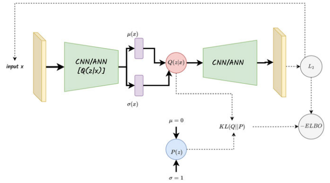
Figure 18. Illustration of a Variational Autoencoder (VAE). This generative model has been extensively used in astronomy for multiple emulation tasks. A first CNN maps the input into a distribution, which is then sampled to provide the input to a second CNN which reconstructs the input image. A regularisation term is added to ensure that the latent distribution behaves close to a prior distribution.
