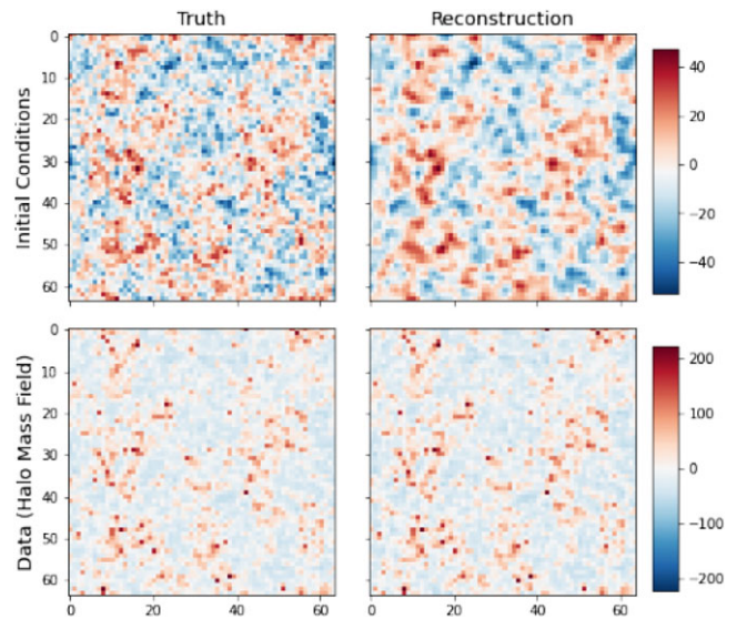
Figure 46. CosmicRIM initial conditions reconstruction technique of Modi et al. (2021a) based on a 3D LSTM recurrent neural network and includes explicitly at each iteration the gradients of the data likelihood. The plot shows a given ground truth initial condition field (top left) and associated final field (bottom left), along with the reconstructed initial conditions (top right) and reconstructed final field (bottom right).
