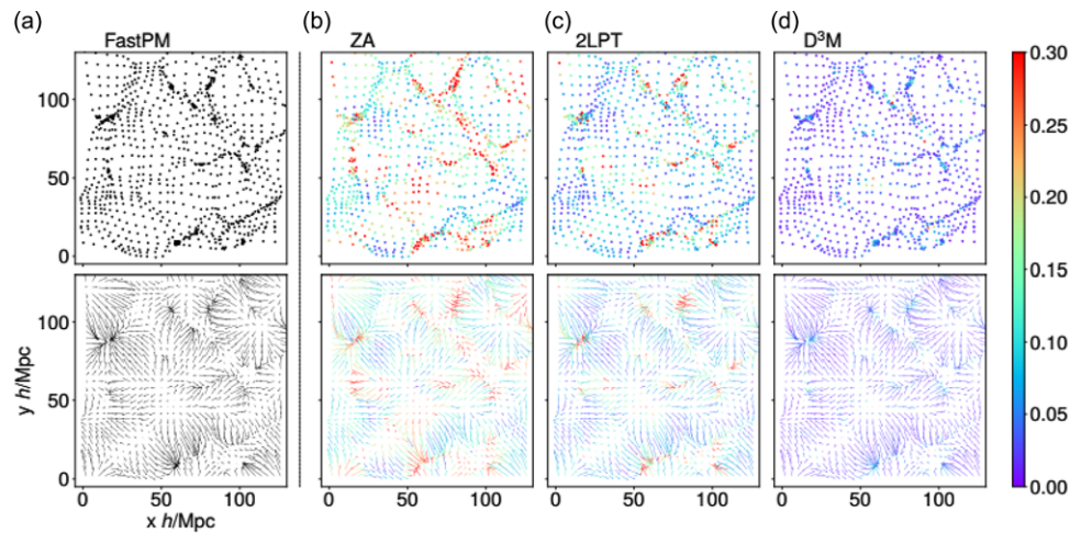
Figure 40. Illustration of learned displacement field in an N-body simulation from He et al. (2018). The first column is the reference simulation (FastPM), the second column shows a simple linear displacement (ZA), the third column shows a second order Lagrangian Perturbation Theory displacement (2LPT) and the last column shows the output of the 3D U-Net (D 3 M). The top row shows final particle positions, the bottom row shows the final displacement field. The colour scale shows the error in position or displacement vectors between each approach and the reference FastPM simulation.
