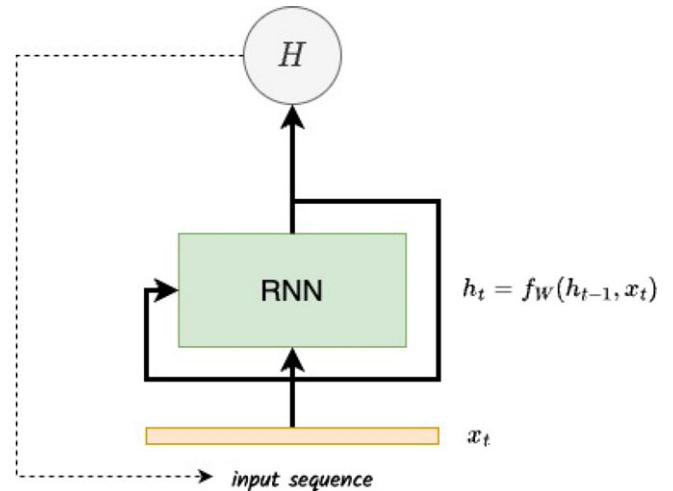
Figure 8. Schematic view of a Recursive Neural Network (RNN) which has been used for classification of light curves in several works. The photometric sequence is fed to a recursive block and trained with a cross-entropy loss. The RNN blocks keep a memory ( h_t ) of the previous time step which make them suitable for handling time sequences.
