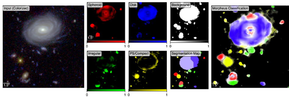
Figure 15. Example of pixel-level classification of a region in the CANDELS survey using a Unet. The leftmost image shows the original field. The six smaller images show different channels with different morphological types and the rightmost image is the combination of all channels with a pixel-level morphological classification. Figure adapted from Hausen & Robertson (2020)
