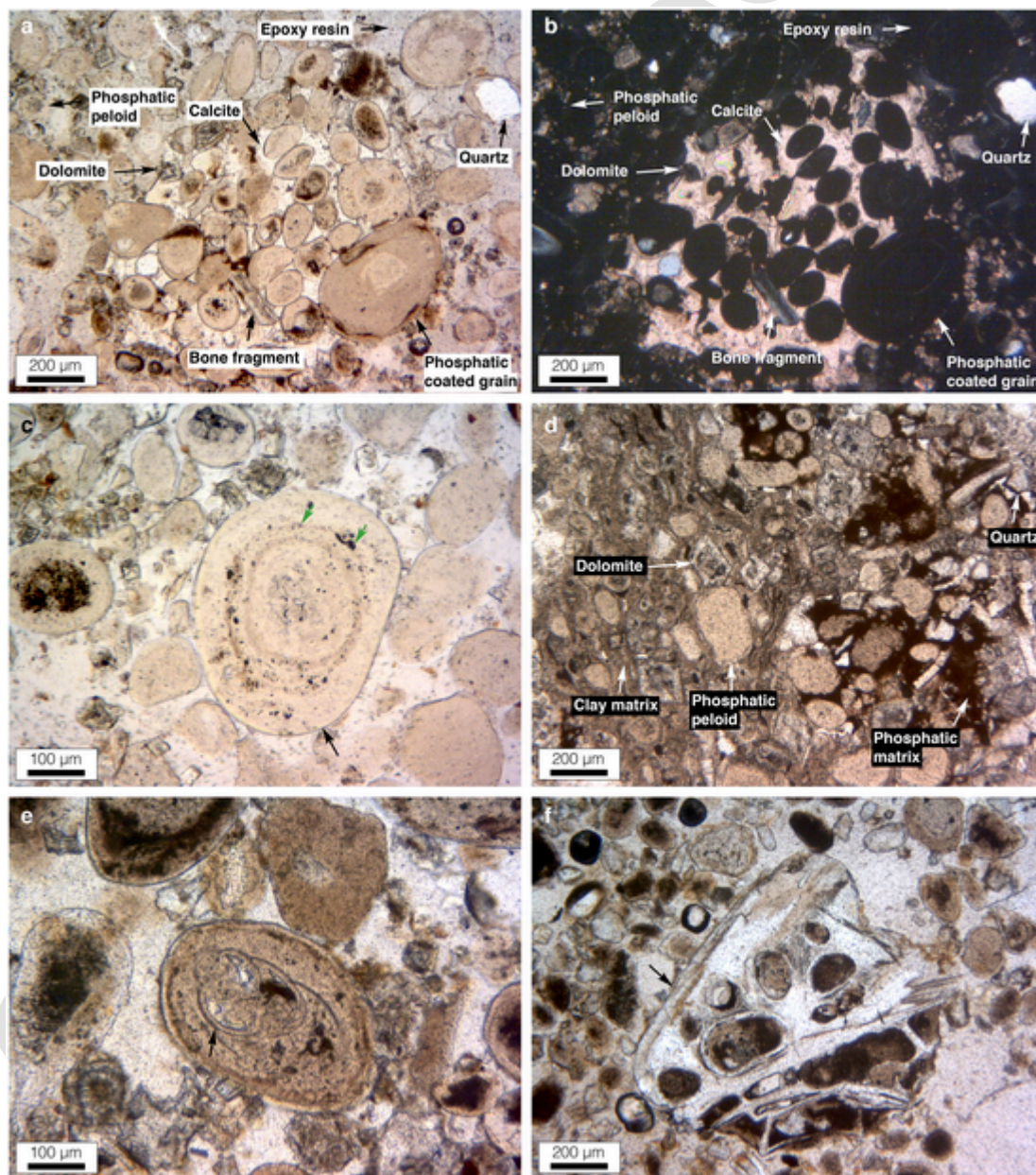
Fig. 2. Photomicrographs of representative phosphatic grains from the 6258 well, Gantour Basin. Images are in plane-polarized (a, c-f) and cross-polarized lights (b). (a, b) Phosphatic peloid and coated grains, bioclasts, as well as detrital quartz grains embedded within a carbonate-dominated matrix. The phosphatic allochems show a large variation in size and shape. (c) Phosphatic coated grain (black arrow) consisting of alternating light-brown and dark-brown laminations. Green arrows denote grain porosity. (d) Heterogeneous phosphatic peloids supported by dolomite as well as clay and phosphatic cements. (e) Phosphatized gastropod shell (black arrow) found as a nucleus within a phosphatic coated grain. (f) Partially phosphatized, mm-long bone fragment (black arrow). (For interpretation of the references to colour in this figure legend, the reader is referred to the web version of this article.)
