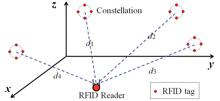
Fig. 1. Constellation approach for localization using multilateration.
