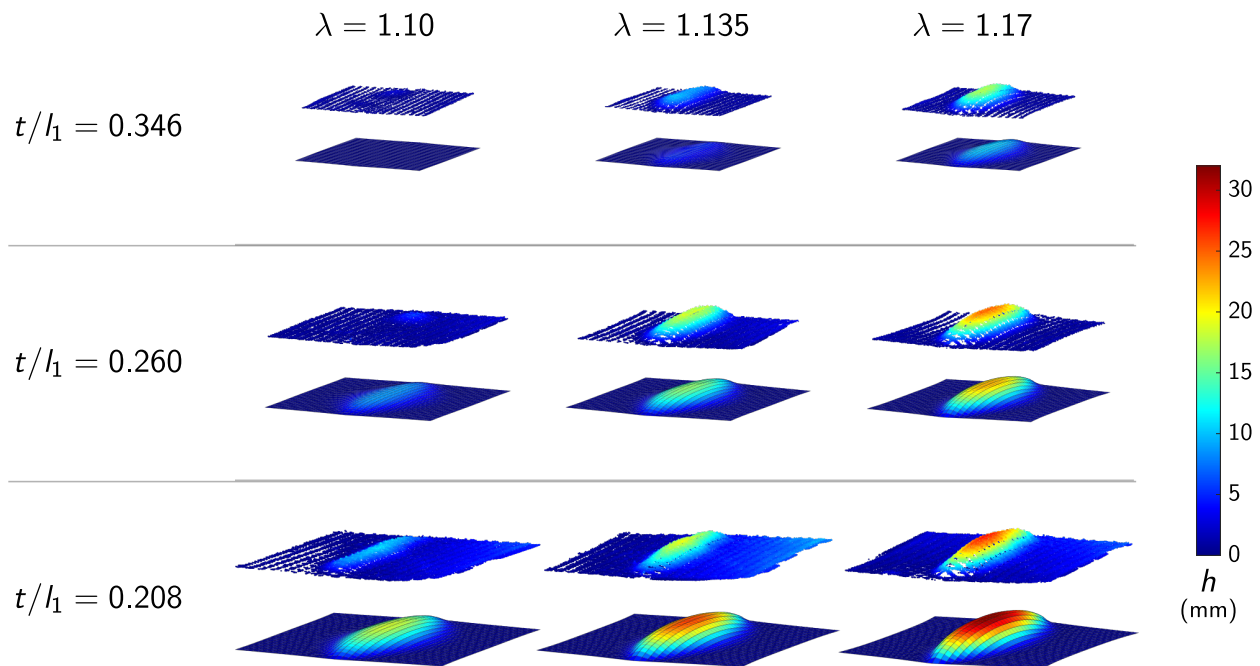
Fig. 6: Post-buckling behavior of sheets with three thickness-to-width ratios. These are the same three sheets represented in Fig. 5c. Here, t is the sheet thickness, l_1 is the length of the unit cell grid spacing in the e_1 direction, and \lambda is the applied stretch at the midpoint of the sheet edge. In each entry of the stretch vs. aspect ratio grid, the laser scans are plotted directly above the simulated deformed meshes. As expected, we see that sheets with higher thickness-to-width ratios will nucleate at larger stretches and will buckle into wider domes relative to the overall sheet width.
