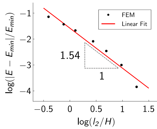
Fig. E.8: Mesh convergence analysis. E is the energy of buckled sheet at a stretch of \lambda = 1.17 for meshes varying from 12 \times 12 to 64 \times 64 . E_{min} is the energy of the sheet when using an 84 \times 84 mesh. H is the element length and l_2 is the characteristic unit cell length. The slope of the linear fit shown in the figure corresponds to the convergence rate.
