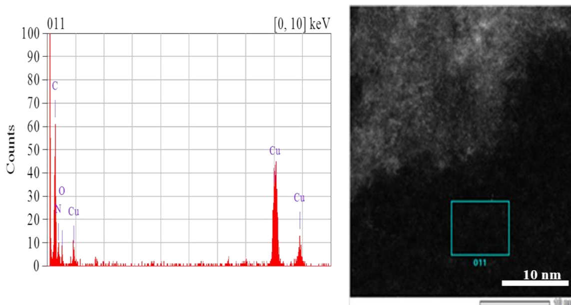
Fig. SI 1: EDX analysis of the boxed area on the right image (scale bar =10 nm) and corresponding to the matrix surrounding the hybrid species
