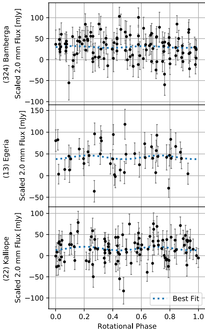
Figure 6. Phased light curves of (324) Bamberga (top panel), (13) Egeria (middle panel), and (22) Kalliope (bottom panel) at 2.0 mm, folded over the rotational period and scaled to mean observed solar distance, Earth distance, and solar phase angle as described in Section 4. The dotted blue lines represent the sinusoidal function that best fits the data, although none of these fits are statistically significant. The sinusoidal periods are constrained to half the rotational periods, but the amplitudes and phases are free parameters.
