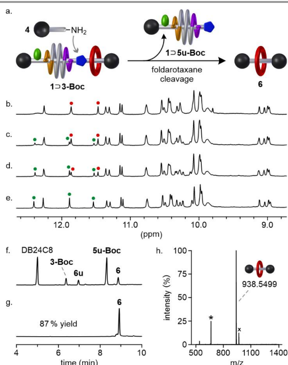
Fig. 4. (a) Cartoon illustrating the aminolysis of 1⊃3-Boc that leads to rotaxane 6. Parts of the ^1\text{H} NMR spectra (700 MHz, 298 K) showing the amide resonances of 1⊃3-Boc (6 mM) in \text{CDCl}_3 : (b) the initial 1⊃3-Boc foldarotaxane; and in the presence of the amine 4 (16.5 mM) after: (c) 1h, (d) 3h30 min and (e) 18h. The resonances of 1⊃3-Boc and 1⊃5u-Boc are marked with red and green circles, respectively. HPLC chromatograms (C8 column, \text{H}_2\text{O} + 0.1\% TFA / \text{MeCN} + 0.1\% TFA - 60:40 to 0:100, 293 K, 254 nm) of: (f) the mixture of the different components obtained after the aminolysis 1⊃3-Boc at the exclusion of 1⊃5u-Boc that has been previously removed by preparative GPC. (g) Rotaxane 6 after purification using silica chromatography. (h) Electrospray ionization mass spectrum (ESI-MS) of the rotaxane 6. The star and the cross denoted an artefact of the mass spectrometer and an undetermined m/z value of [6 + 28], respectively.
