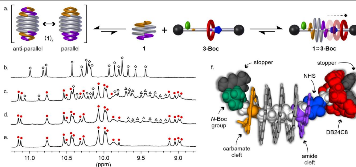
Figure 3. (a) (left) Equilibrium between double helix ( 1 ) 2 and single helix 1 . Note that, as sequence 1 is dissymmetrical, ( 1 ) 2 can be either parallel or antiparallel. (right) The formation of the foldarotaxane 1 → 3-Boc requires the unfolding and refolding of the helix around the molecular axle. The binding of 1 forces the translocation of the macrocycle (DB24C8) through the NHS moiety (blue pentagon). (b-e) Kinetic monitoring of the folding of single helix 1 (6 mM) around axle 3-Boc (15 mM) in CDCl 3 followed by 1 H NMR (700 MHz, 298 K) and showing the amide resonances of the helix; (b) initial single helix 1 ; (c) 18 h after the addition of 3-Boc ; then after (d) 72 h and (e) 144 h. For the equilibration procedure see the ESI. Amide signals of 1 , ( 1 ) 2 and 1 → 3-Boc are marked with diamonds, triangles and red circles, respectively. (f) Energy-minimized molecular model, built using MMFFs of the foldarotaxane 1 → 3-Boc . The various functional groups are colour coded as in Figure 1. Side chains and non-polar hydrogen atoms of the helix have been removed for clarity.
