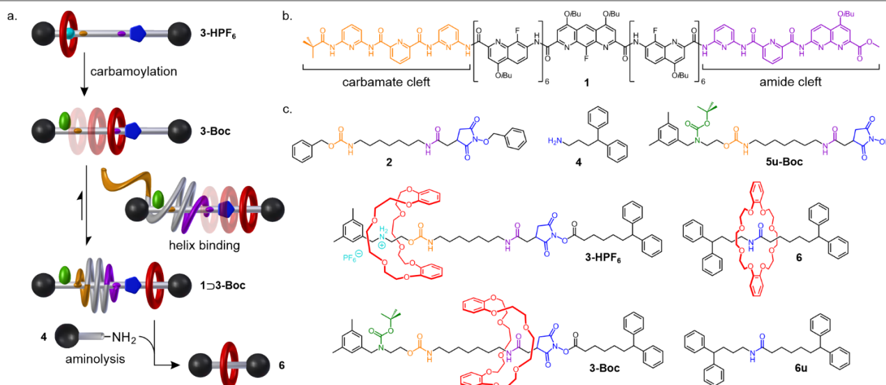
Fig. 1. (a) Schematic representation of the successive molecular machineries, first between the [2]rotaxanes 3-HPF 6 and 3-Boc through deprotonation-then-carbamoylation of the ammonium, then by the displacement and sequestration of the DB24C8 after the entwining of the helix to produce a foldarotaxane. The helix binding induces the displacement of the macrocycle that becomes sequestered on a part of the axle for which it has no affinity. It follows that the cleavage of the axle can yield a [2]rotaxane. (b) Sequence of the dissymmetrical helix 1 and (c) formulae of rotaxanes 3-HPF 6 , 3-Boc and 6 and non-interlocked molecular axes and reactants 2 , 4 , 5u-Boc and 6u .
