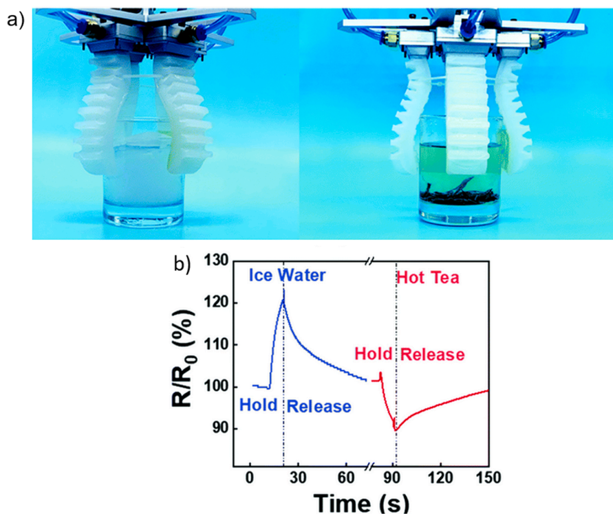
Fig. 13. (a) Photos of the soft gripper with integrated SSHTS based on a hydrogel and poly-ionic liquids holding a cup of ice water and a hot tea (approximately 60 °C); (b) the resistive signal of the holding process. Reproduced with permission from [277].
