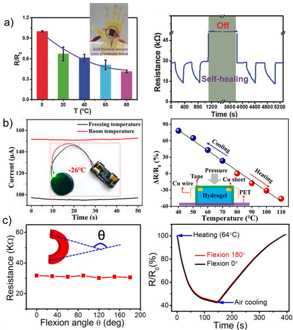
Fig. 8. (a) A 2 \times 2 cm 2 soft thermal sensor, based on single-wall CNTs, was used to measure the temperature between 0 and 80° on a soft prosthetic hand. Thermal sensitivity was investigated at different temperatures (0, 20, 40, 60, and 80 °C) and the resistivity before damage and after healing. Reproduced with permission from [193]. (b) A PAAni/PAA hydrogel thermistor was investigated under different thermal conditions, with a voltage of 3 V. Reproduced with permission from [179]. (c) Double network hydrogel based on PAAm and \kappa -CA was used as a flexible electronic conductor for LED application. The sensor device was tested at different flexion angles and under thermal heat treatment. Reproduced with permission from [194].
