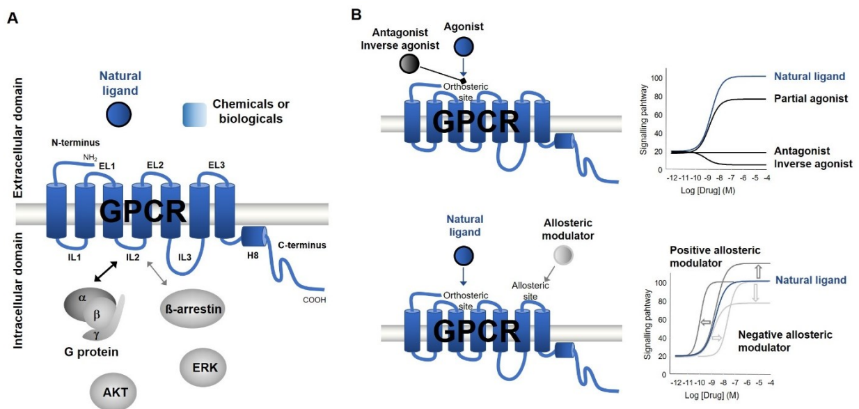
Figure 1 GPCR signalling and pharmacology
