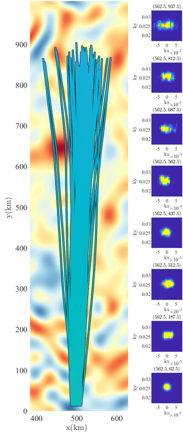
Fig. 3: Swell interacting with a low-resolution ( 32 \times 32 ) deterministic SQG current plus (one realization of) the time-uncorrelated stochastic model. Ray trajectories are computed by forward advection and superimposed on the low-resolution current vorticity \bar{\omega} = \nabla^\perp \cdot \bar{\mathbf{v}} .
