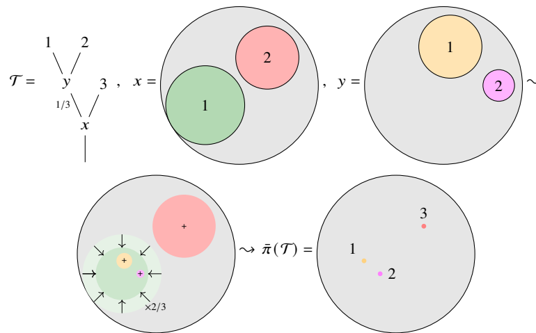
Fig. 5.8 Construction of the morphism \tilde{\pi} : WD_n \rightarrow FM_n .
