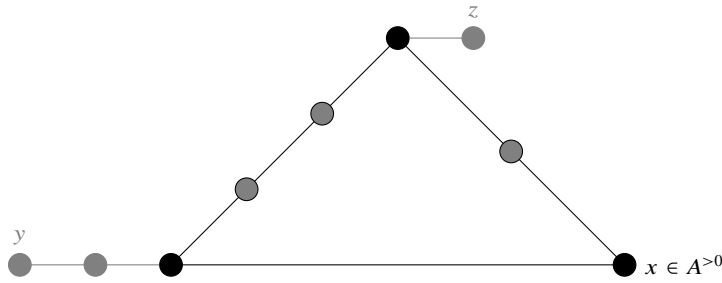
Fig. 3.6 A graph and its core (in black).
