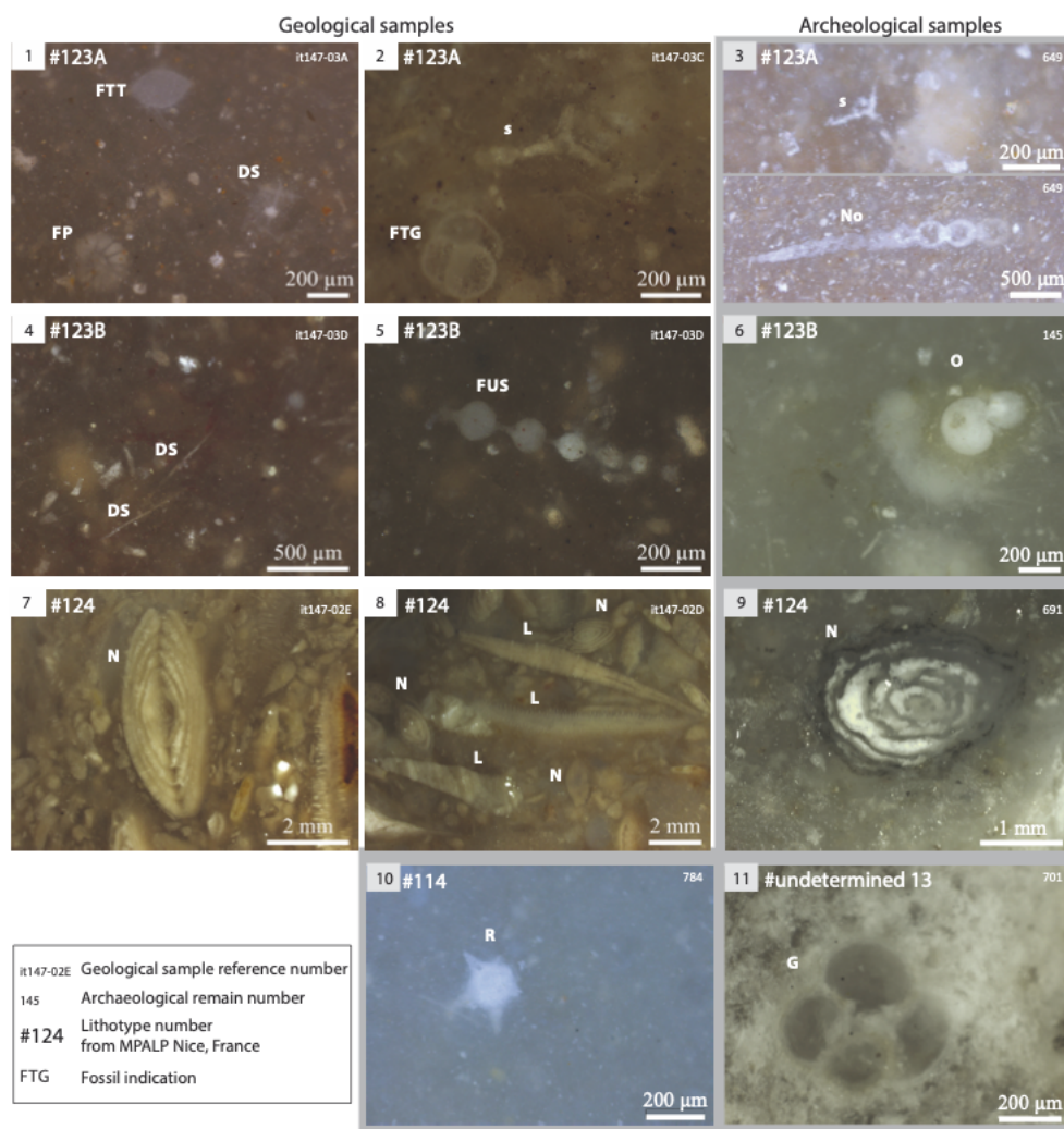
Fig. 4 - Description and pictures of the cherts lithotypes identified in geological and archaeological samples from Valle Giumentina (stereomicroscope, reflected light). 1, FTT: Foraminifera, trochospiraled test with trapezoids chambers; FP: Foraminifera planispiraled test; DS: Deteriorated spicule. 2, FTG: Foraminifera, trochospiraled test with globular chambers; S: Spicule. 3, No: Nodosoria; S: Spicule. 4, DS: Deteriorated spicules remains identifiable. 5, FUS: Foraminifera, uniserial test with spherical chambers. 6, O: Orbulinae. 7, N: Nummulitidae. 8, L: Lepidorbitoidae; N: Nummulitidae. 9, N: Nummulitidae. 10, #114 refers to the Maiolica chert, not available in the Maiella mountain; R: Radiolaria. 11, G: Globigerinidae. (Pictures : A. Tomasso, CAD: E. Nicoud).
