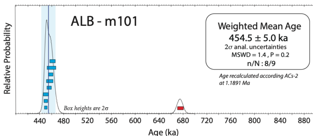
Fig. 6 - ^{40}\text{Ar}/^{39}\text{Ar} dating of cryptotephra identified in layer ALB-42 of Valle Giumentina (sample m101). Probability age diagram obtained.
