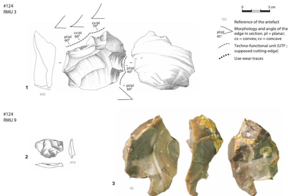
Fig. 13 - Flake industry from Valle Giumentina ALB-42 (RMU #124-3 and 9). 1, thick flake with a notched edge. 2, small retouch flake. 3, thick plunging flake. (Ink drawings by M. Pagli; pictures and CAD: E. Nicoud).
