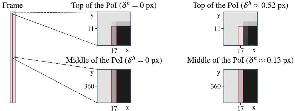
Figure 2: Edge pixels of interest for displacement estimation, with PoI in red.
