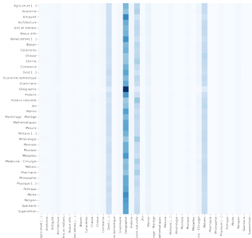
(a) C^2
