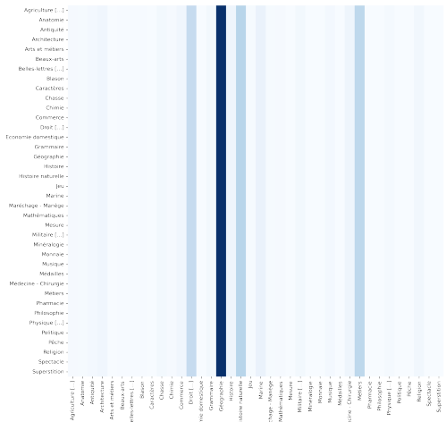
(c) C^{50}
