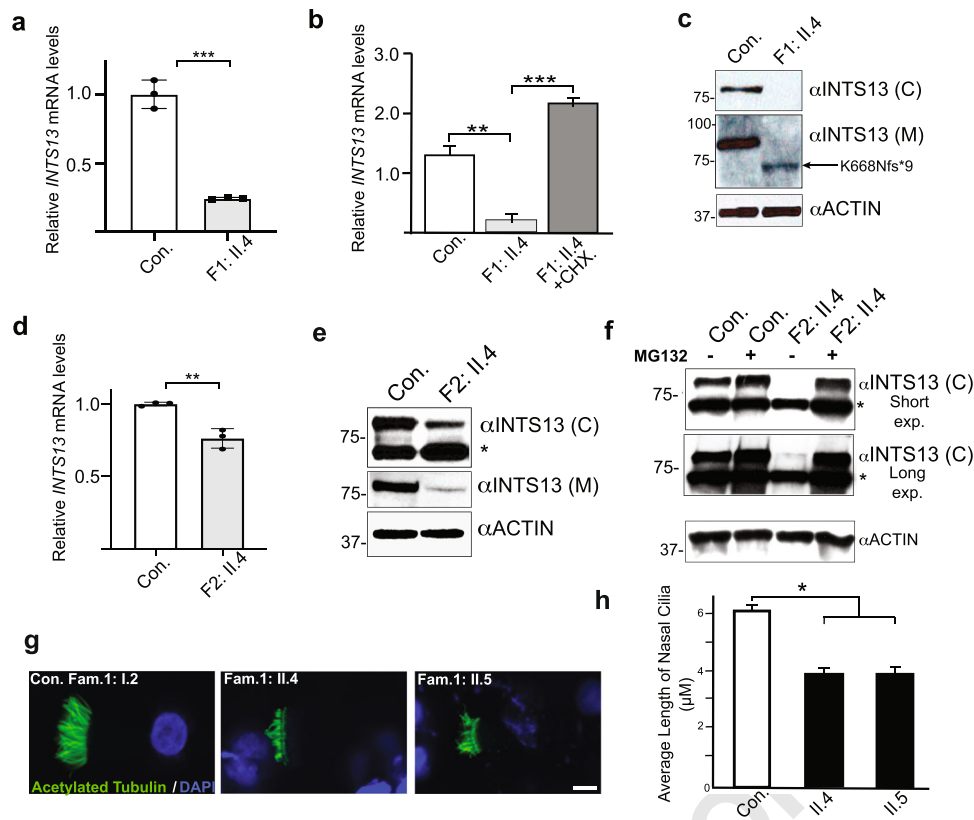
Fig. 2 | Characterization of INTS13 variants using patients' cells. a RT-qPCR shows that endogenous INTS13 transcript levels were significantly reduced relative to control cells in primary dermal fibroblasts of affected individual II.4 from Family 1. Data are mean \pm SD, n = 3 replicate cell samples. Statistical significance was calculated using a two-tailed unpaired t -test. p = 0.000223 . b Primary dermal fibroblasts were treated with cycloheximide (CHX) (100 \mu g/ml). Following treatment, qRT-PCR was done at 8 h and shows that INTS13 mRNA level was increased in treated cells indicating a non-sense mediated decay. Data are mean \pm s.e.m., *P < 0.05 ; **P < 0.005 ; ***P < 0.001 ; one-tailed Student's t -test. c Western blot analysis of primary dermal fibroblasts of affected individual II.4 from Family 1 using two polyclonal antibodies with antibody directed against the C-terminus of INTS13 (C) and the second antibody directed against the center of INTS13 (M). Actin was used as a loading control and molecular weight markers shown are in kilodaltons. d RT-qPCR shows that INTS13 transcript levels were significantly reduced in primary dermal fibroblast cells of affected individual II.4 from Family 2 relative to control
