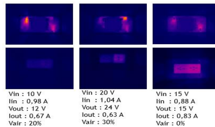
Fig 5. IR images from Fluke camera of a DC/DC converter operating in different operating points, T_a=23^{\circ}C
