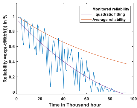
Fig 9. The reliability monitored for the inductance vs the average mission profile reliability
