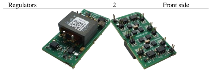
Fig 7. G2Elab DC/DC DAB converter, on the left the front side, on the right of the backside.
