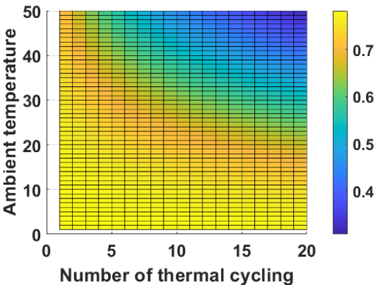
Fig 4. Color map of the theoretical MTBF of a wound inductor versus the ambient temperature and the number of thermal cycles.
