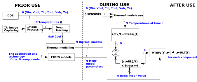
Fig 6. The process of data collection and calculation to obtain the MTBF from the operating points.
