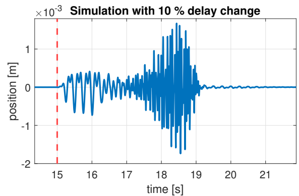
Fig. 7. Response to 10 % delay change after 15 seconds of simulation.
