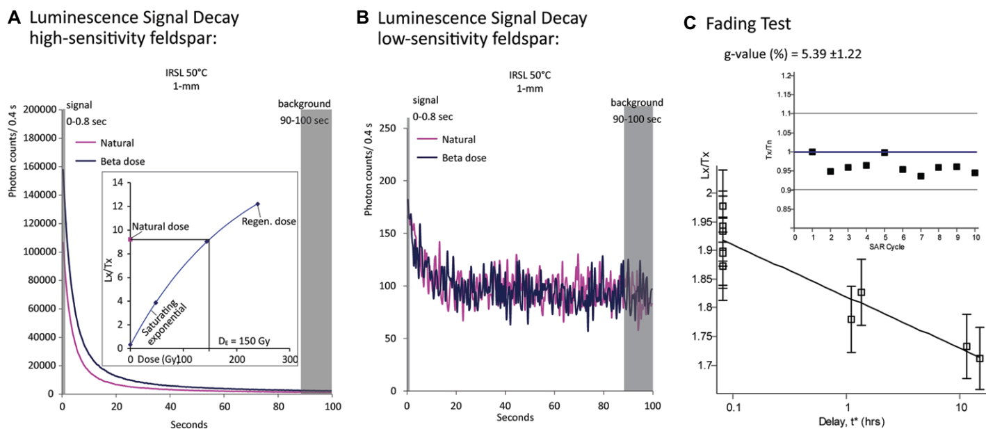
Figure 8. Characteristic feldspar luminescence properties are shown. (A) Luminescence Signal Decay: high-sensitivity feldspar IRSL 50 °C on 1-mm small aliquot (~10 grains). The inset dose response curve is well below saturation. (B) Luminescence Signal Decay: low-sensitivity feldspar IRSL 50 °C on 1-mm small aliquot (~10 grains). (C) Fading Test results of nine sensitivity-corrected dose cycles with varying measurement delays following Auclair et al. (2003).
