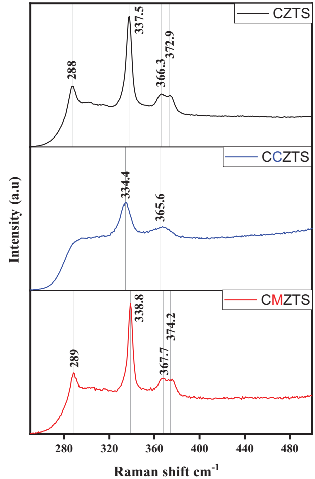
Fig. 3. Raman spectra for CZTS, CCZTS and CMTS samples.
