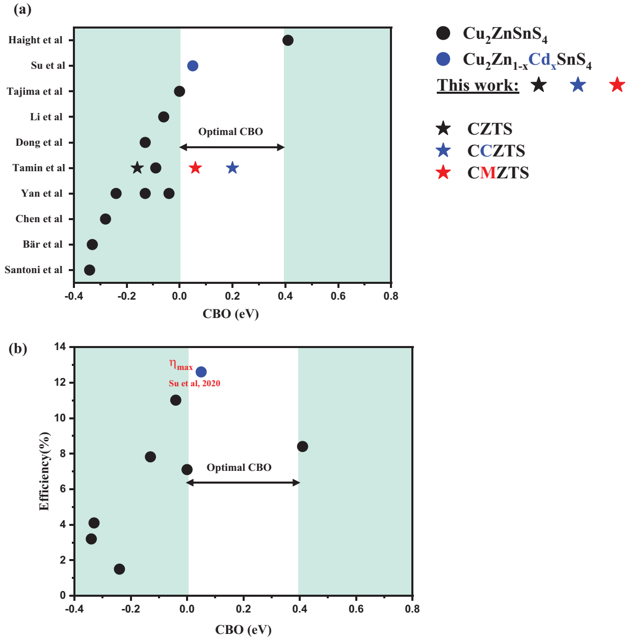
Fig. 7. (a) An overview of all the experimental work reported in the literature on the CBO value of pure sulfide kesterite. (b) An overview of the performance of solar cells based on pure sulfide in the literature as a function of CBO value.
