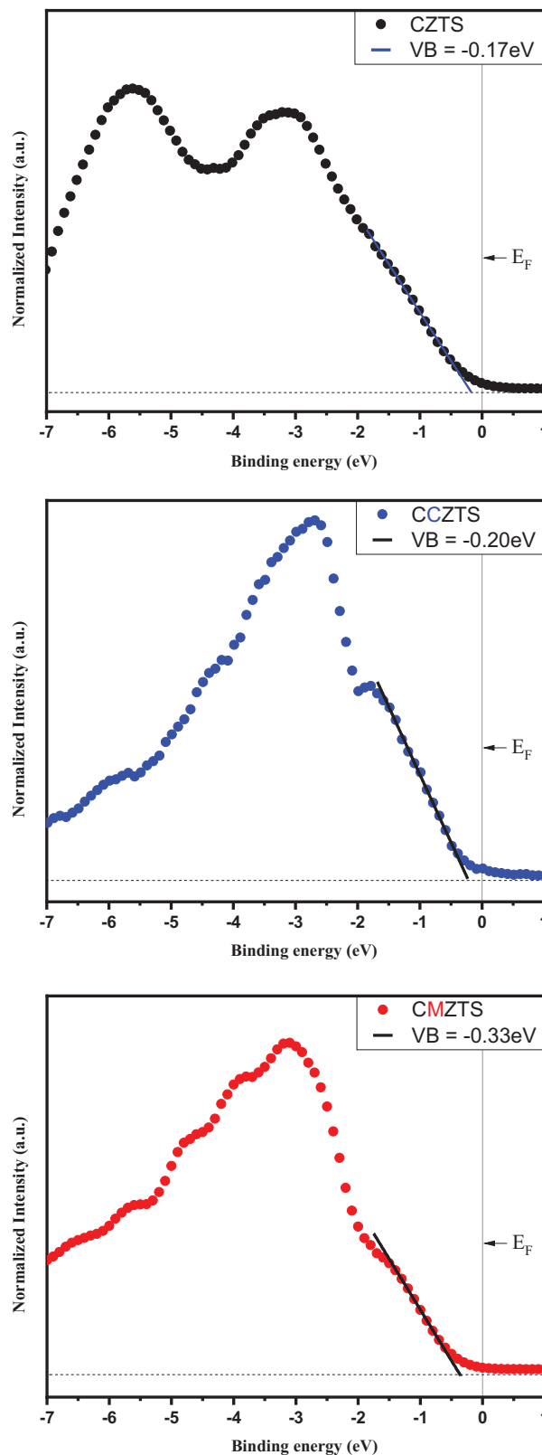
Fig. 5. Estimation of the valence band position from XPS measurement. (a) CZTS, (b) CCZTS, (c) CMZTS.
