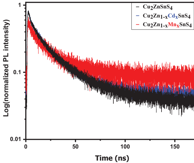
Fig. 10. Normalized and time-resolved photoluminescence decay with excitation wavelengths of 488 nm. Black color CZTS/CdS, blue color CCZTS/CdS and red color CMZTS/CdS.
