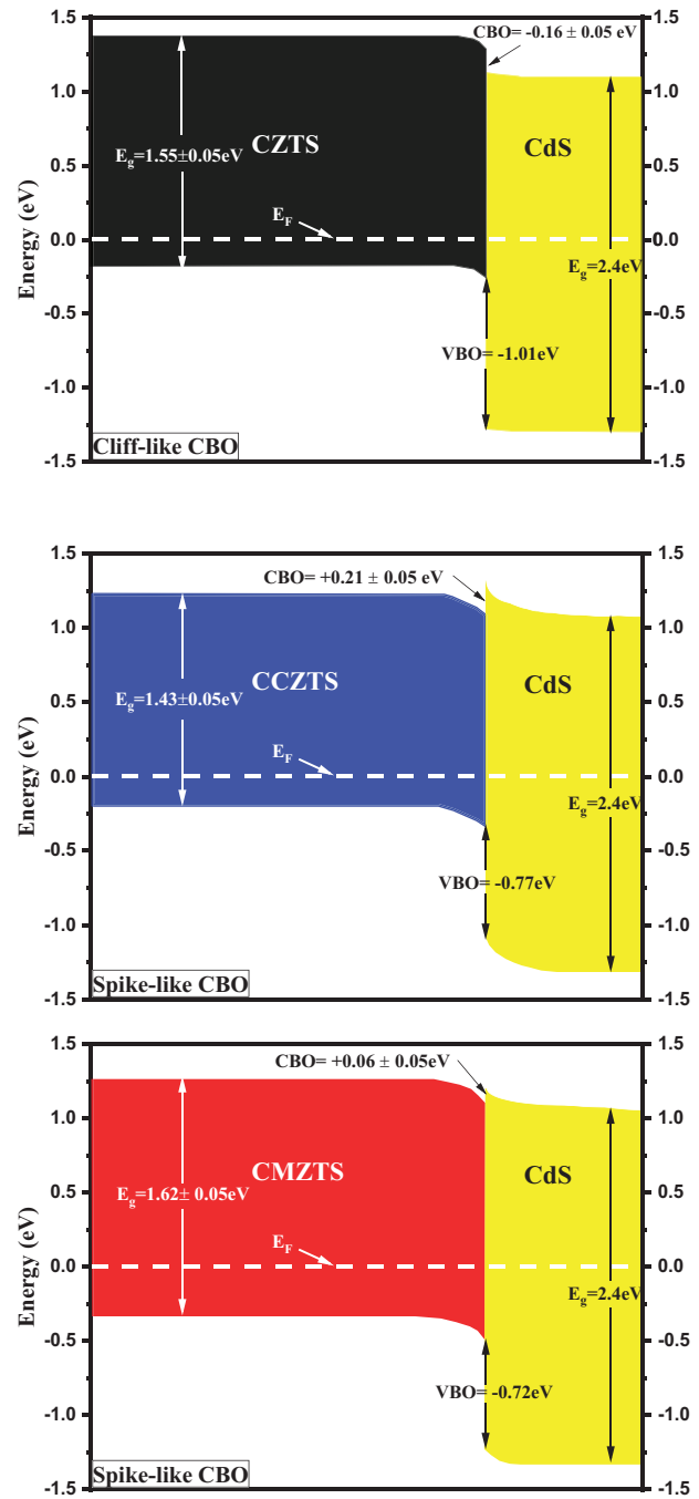
Fig. 9. Experimental band alignment at absorber/buffer hetero-junction. (a) CZTS/CdS, (b) CCZTS/CdS, (c) CMZTS/CdS.
