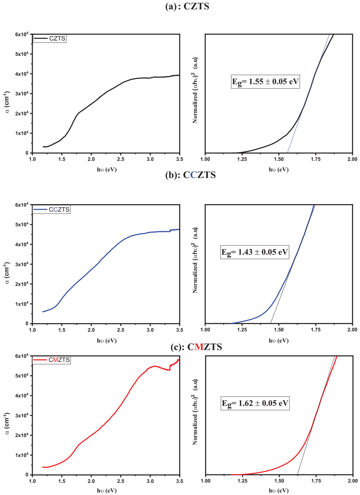
Fig. 4. Estimation of the band gap and the absorption coefficient from the UV/Visible measurement. (a) CZTS, (b) CCZTS, (c) CMZTS.
