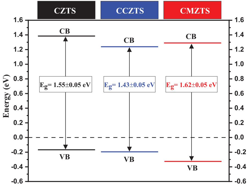
Fig. 6. Valence and conduction band positions of CZTS, CCZTS and CMZTS.
