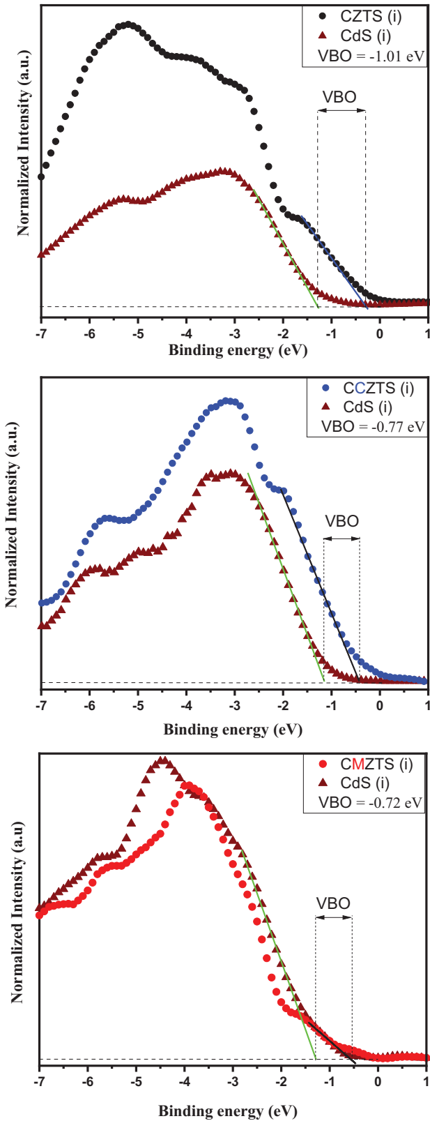
Fig. 8. Estimation of VBO at the absorber/buffer hetero-interface by direct XPS measurement. (a) CZTS/CdS, (b) CCZTS/CdS, (c) CMZTS/CdS.
