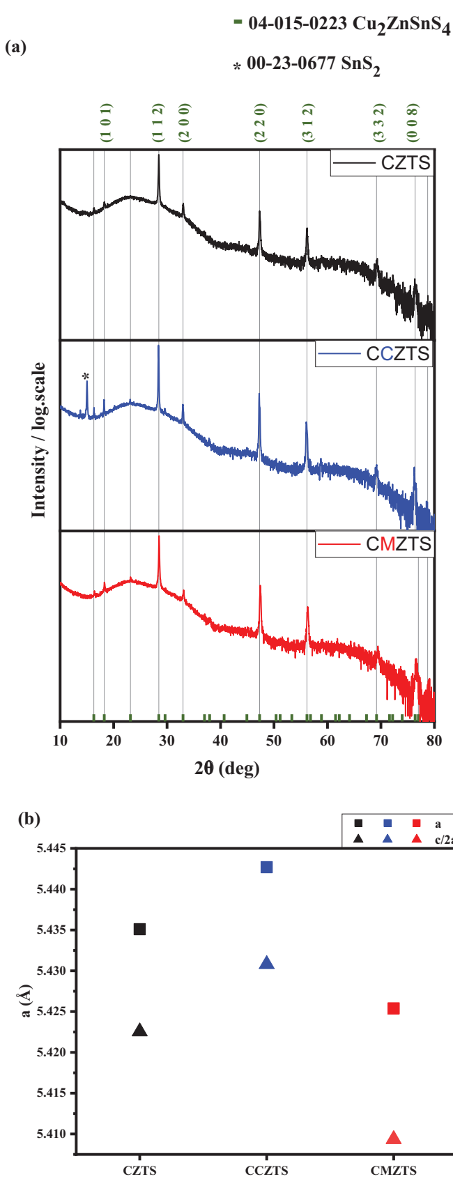
Fig. 2. X-ray diffractogram (a) and lattice parameters (b) of CZTS, CCZTS and CMZTS samples.
