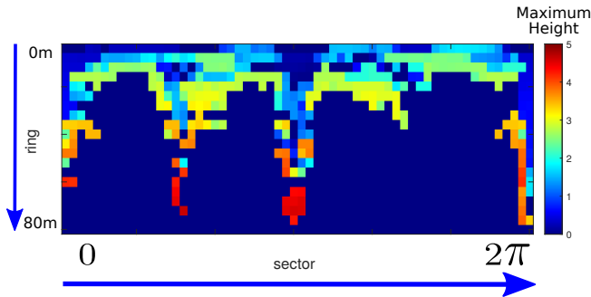
Figure 2: Illustration of the Scan Context.
