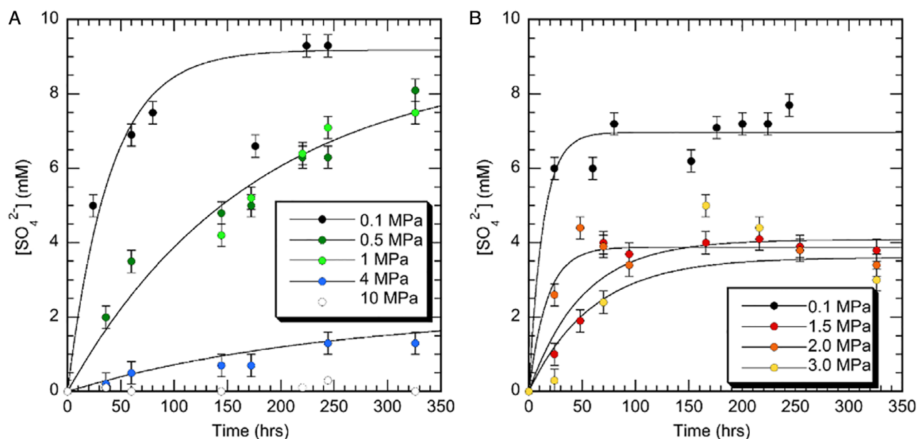
Fig. 2. Kinetics of sulfate production by T. thioparus as a function of pressure to 10 MPa with different initial concentrations of thiosulfate [S_2O_3^{2-}]_0 ranging from 5 g.l -1 (A) to 15 g.l -1 (B).
