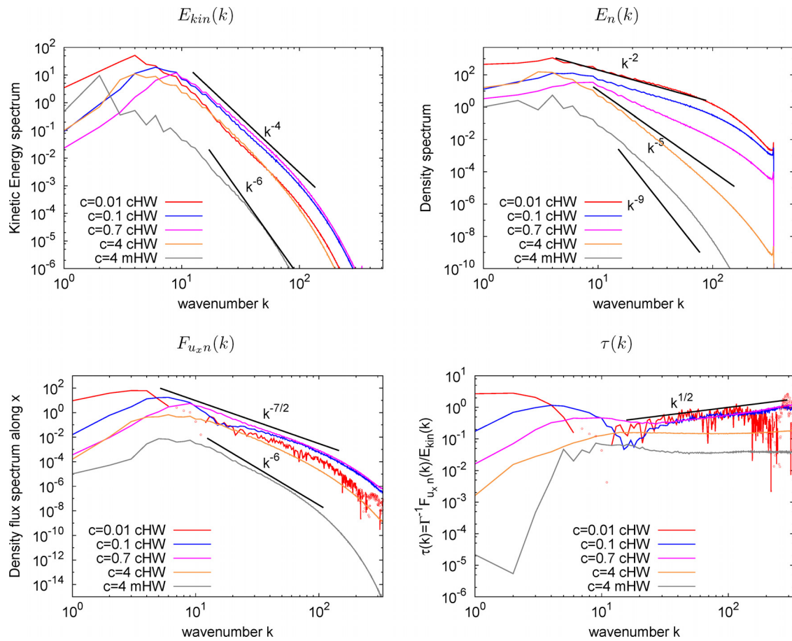
FIG. 3. Top: Eulerian kinetic energy spectra E_{kin}(k) (left) and Eulerian spectra E_n(k) of density fluctuations (right). Bottom: density flux spectra F_{u_x n}(k) (left) and spectral timescale \tau(k) = \Gamma^{-1} |F_{u_x n}(k)| / E_{kin}(k) (right). All the spectra are obtained using time-averaging with 75 snapshots taken at regular time intervals in the statistically stationary regimes. Dots in the spectra indicate negative values, plotted by taking the absolute value.
