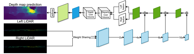
Fig. 3: Modified part of the depth estimation of the SLS-Fusion algorithm to adapt it for using only the LiDAR as input.
