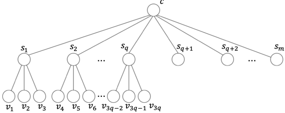
Figure 2: A solution T of the \text{SpHRP} after the reduction.
