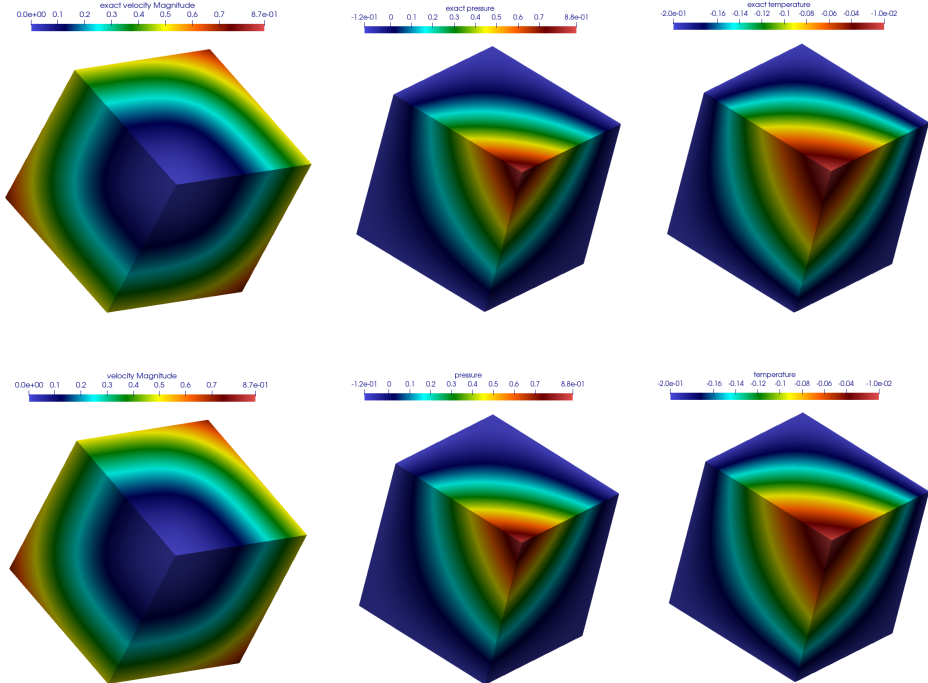
Figure 6: Isovalues of the exact solutions (top) and computed solutions (bottom) using \mathbb{P}_1 finite element spaces for each variable, in a mesh with 24,576 elements; velocity (left), pressure (medium) and temperature (right).
