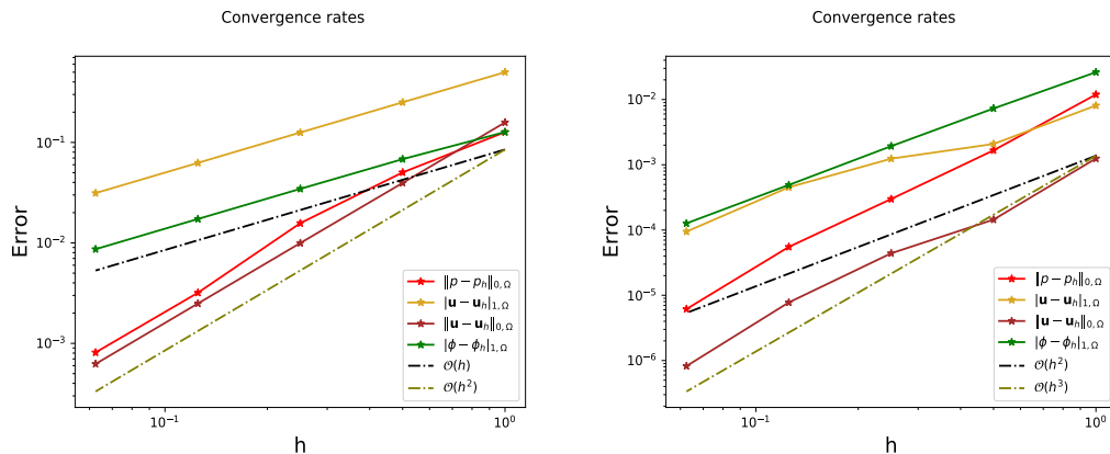
Figure 7: Convergence plots obtained using \mathbb{P}_1 (left) and \mathbb{P}_2 (right) polynomial spaces.
