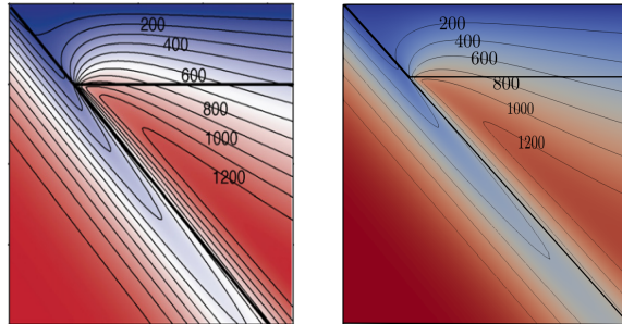
Figure 5: Close up of the model with dislocation creep. Benchmark results introduced in [38] (left) and results using the proposed stabilized scheme (right).
