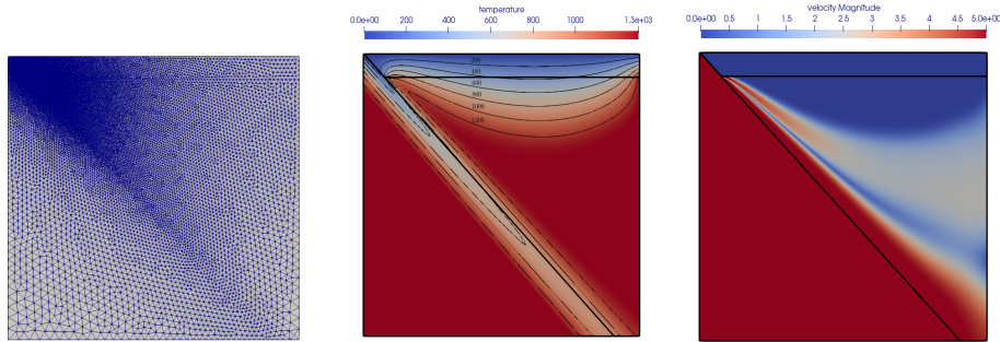
Figure 4: Mesh (left), temperature (middle) and magnitude of the velocity field (right).
