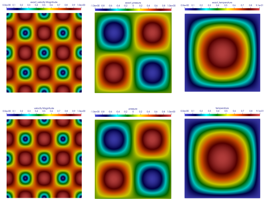
Figure 1: Isolines of exact solutions (top) and computed solutions (bottom) using \mathbb{P}_1 finite element spaces for each variable, in a mesh with 32,768 elements; velocity magnitude (left), pressure (medium) and temperature (right).
