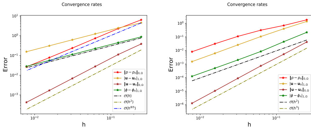
Figure 2: Convergence plots obtained using \mathbb{P}_1 (left) and \mathbb{P}_2 (right) polynomial spaces.
